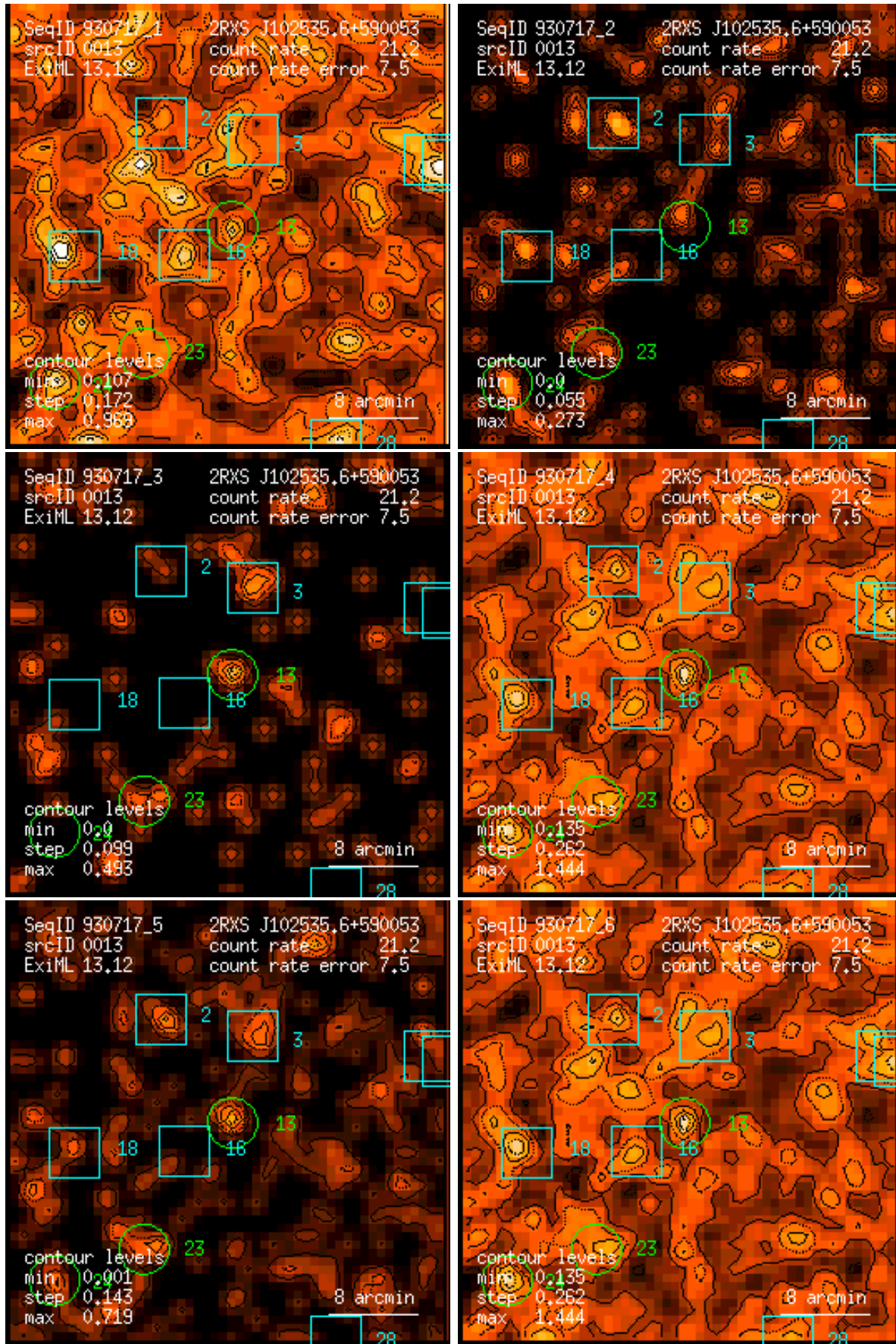
Figure 13: RASS 930717: detection 0013: band rate images, Gaussian filter: (1) PSPC channels 11 – 41, (2) 52 – 90, (3) 91 – 201, (4) 11 – 235, (5) 52 – 201, (6) 11 – 201. Broad band rates in counts/ks. Band rate contour levels in counts/ks/arcmin 2 .
