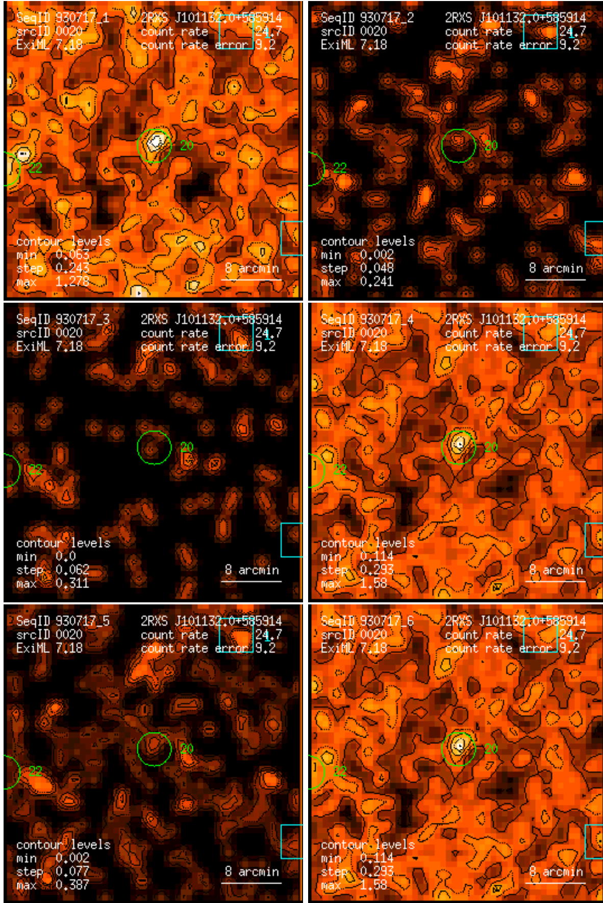
Figure 20: RASS 930717: detection 0020: band rate images, Gaussian filter: (1) PSPC channels 11 – 41, (2) 52 – 90, (3) 91 – 201, (4) 11 – 235, (5) 52 – 201, (6) 11 – 201. Broad band rates in counts/ks. Band rate contour levels in counts/ks/arcmin 2 .
