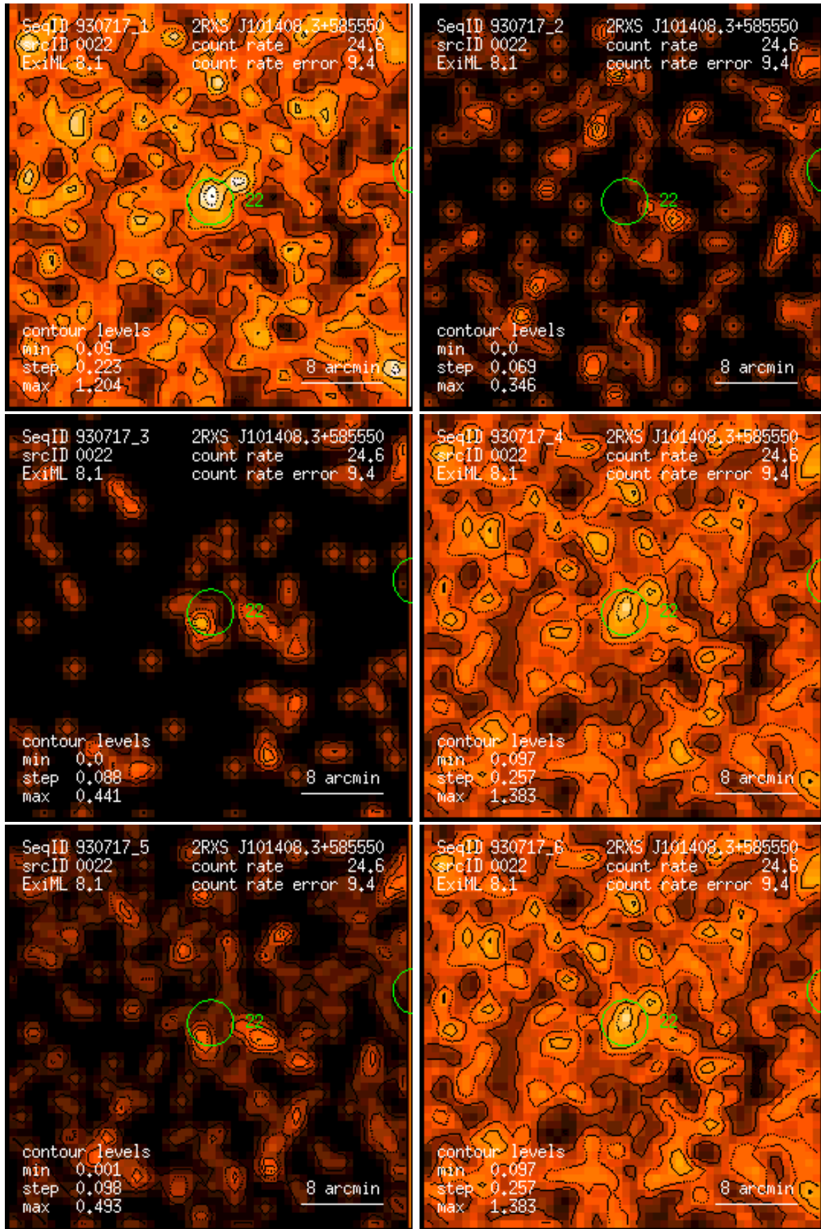
Figure 22: RASS 930717: detection 0022: band rate images, Gaussian filter: (1) PSPC channels 11 – 41, (2) 52 – 90, (3) 91 – 201, (4) 11 – 235, (5) 52 – 201, (6) 11 – 201. Broad band rates in counts/ks. Band rate contour levels in counts/ks/arcmin 2 .
