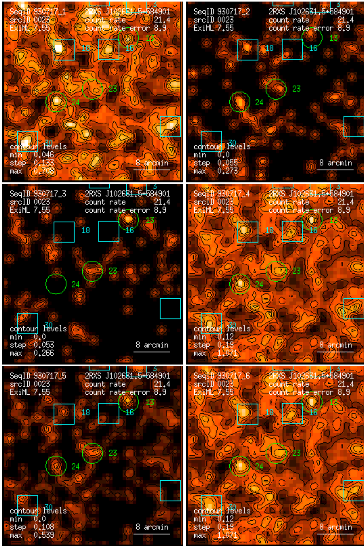
Figure 23: RASS 930717: detection 0023: band rate images, Gaussian filter: (1) PSPC channels 11 – 41, (2) 52 – 90, (3) 91 – 201, (4) 11 – 235, (5) 52 – 201, (6) 11 – 201. Broad band rates in counts/ks. Band rate contour levels in counts/ks/arcmin 2 .
