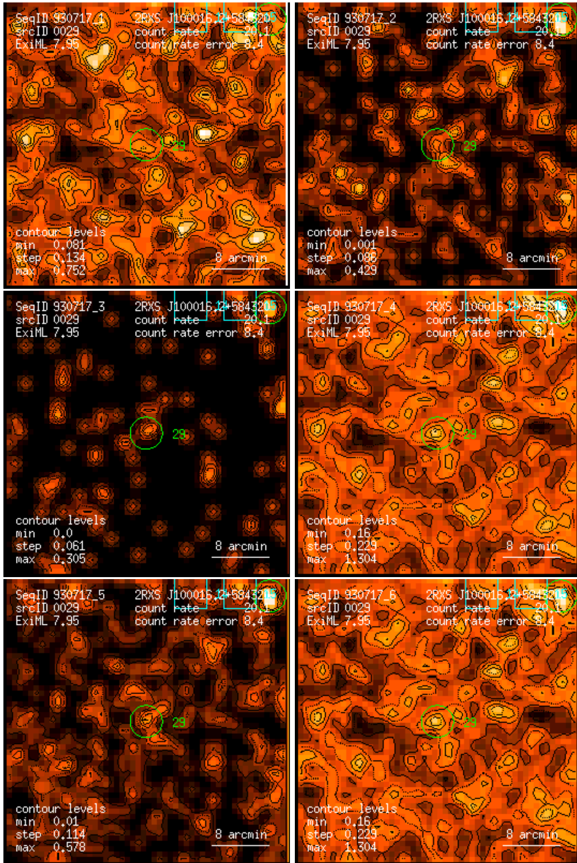
Figure 29: RASS 930717: detection 0029: band rate images, Gaussian filter: (1) PSPC channels 11 – 41, (2) 52 – 90, (3) 91 – 201, (4) 11 – 235, (5) 52 – 201, (6) 11 – 201. Broad band rates in counts/ks. Band rate contour levels in counts/ks/arcmin 2 .
