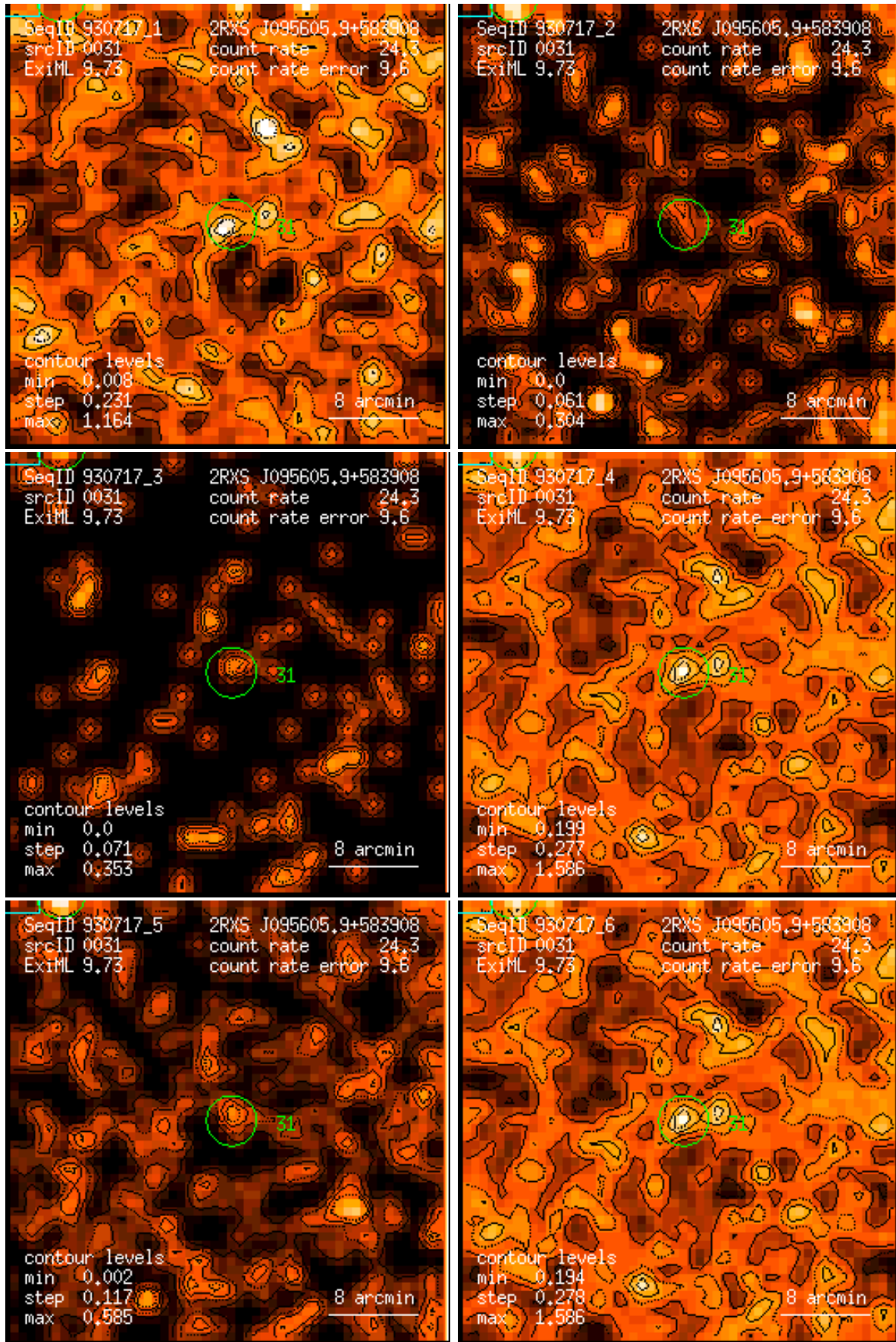
Figure 31: RASS 930717: detection 0031: band rate images, Gaussian filter: (1) PSPC channels 11 – 41, (2) 52 – 90, (3) 91 – 201, (4) 11 – 235, (5) 52 – 201, (6) 11 – 201. Broad band rates in counts/ks. Band rate contour levels in counts/ks/arcmin 2 .
