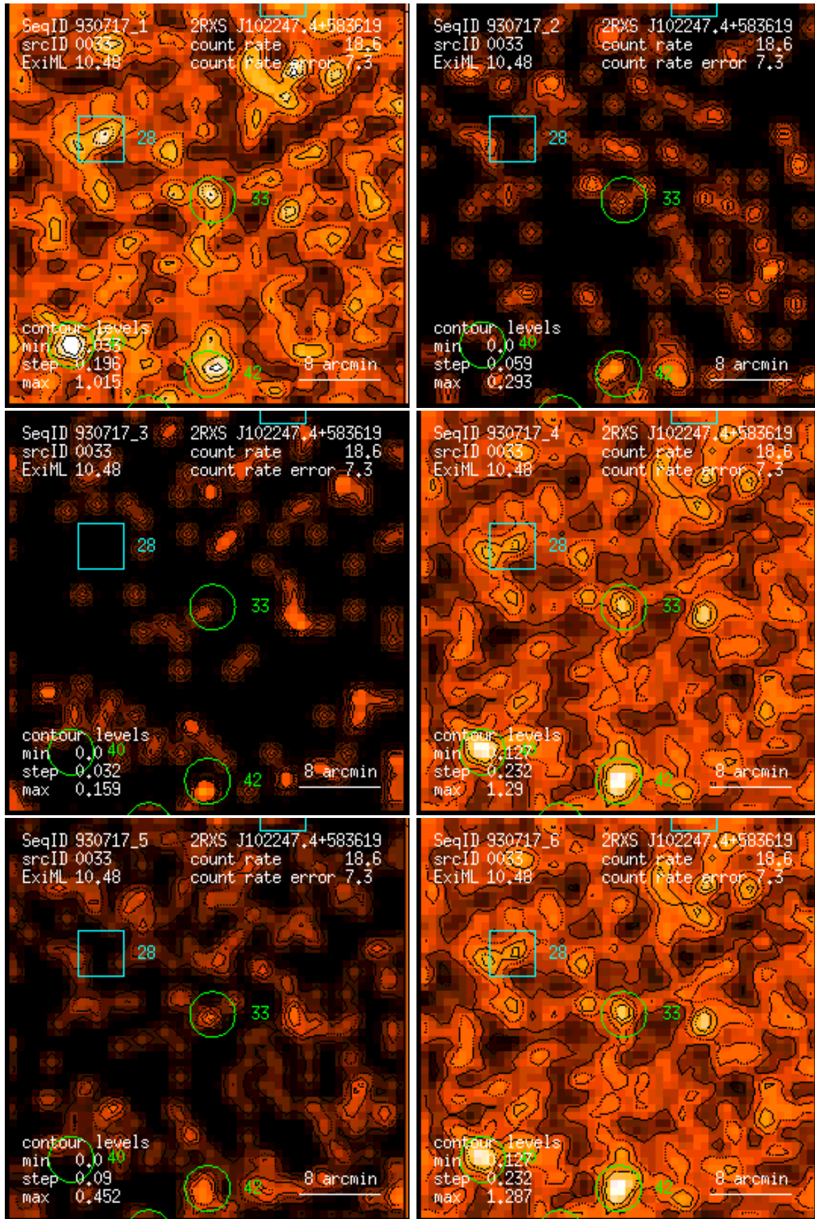
Figure 33: RASS 930717: detection 0033: band rate images, Gaussian filter: (1) PSPC channels 11 – 41, (2) 52 – 90, (3) 91 – 201, (4) 11 – 235, (5) 52 – 201, (6) 11 – 201. Broad band rates in counts/ks. Band rate contour levels in counts/ks/arcmin 2 .
