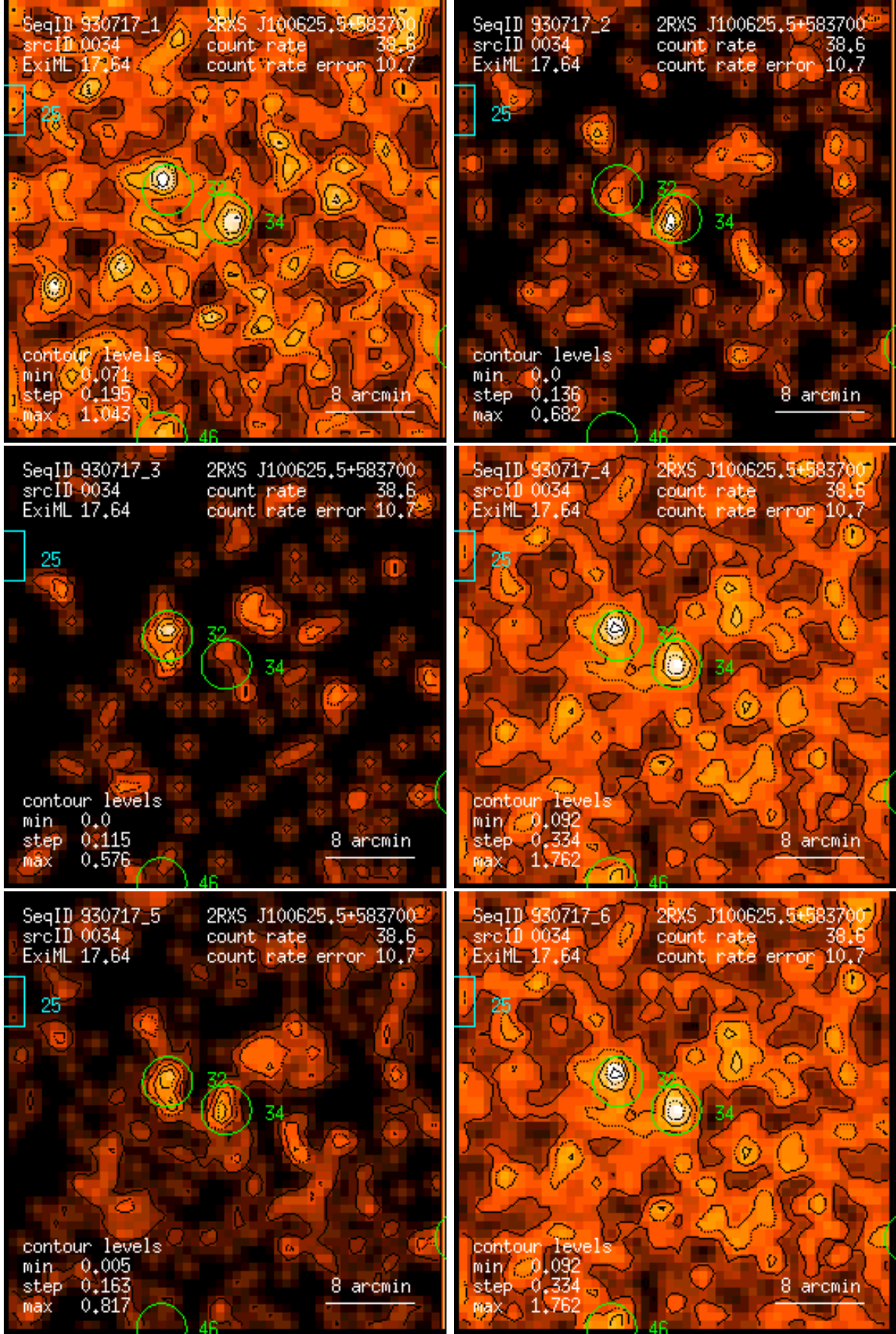
Figure 34: RASS 930717: detection 0034: band rate images, Gaussian filter: (1) PSPC channels 11 – 41, (2) 52 – 90, (3) 91 – 201, (4) 11 – 235, (5) 52 – 201, (6) 11 – 201. Broad band rates in counts/ks. Band rate contour levels in counts/ks/arcmin 2 .
