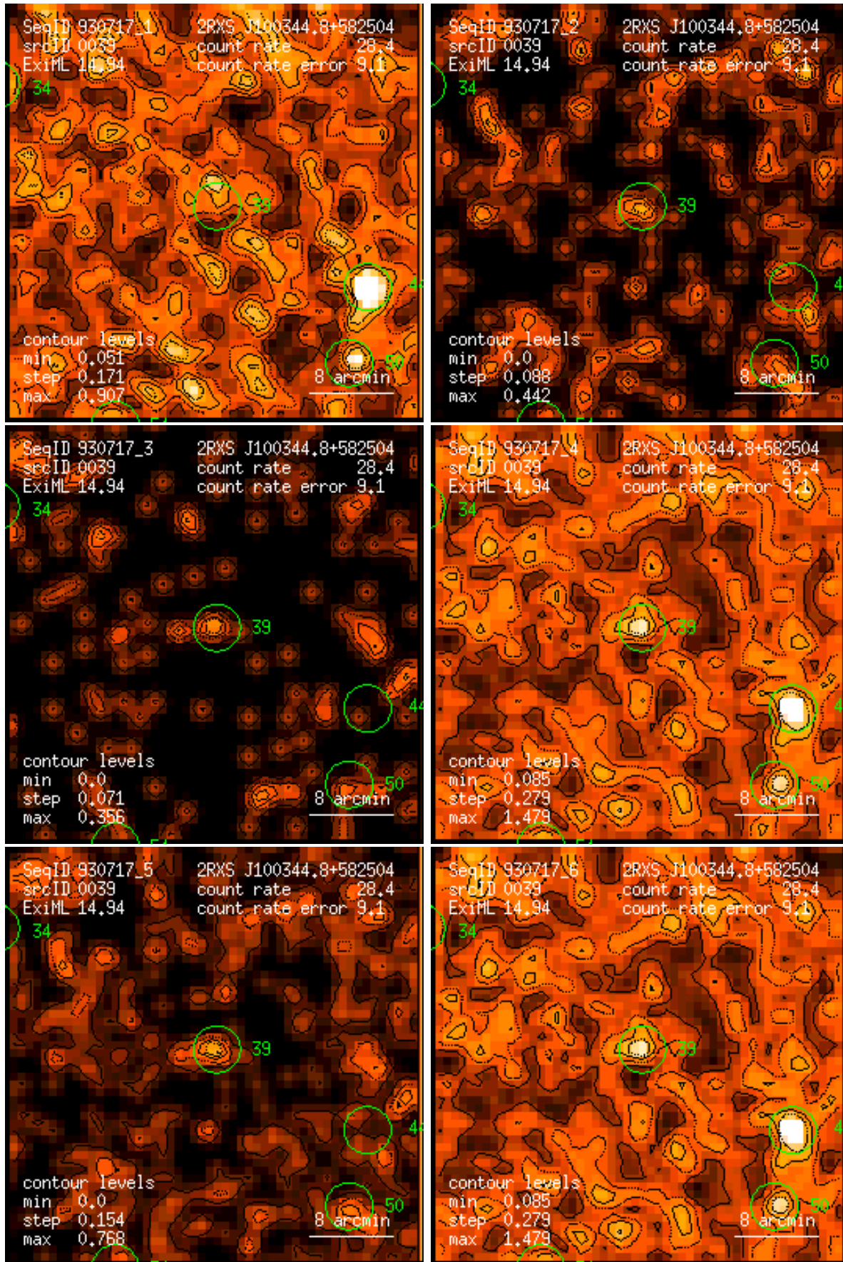
Figure 39: RASS 930717: detection 0039: band rate images, Gaussian filter: (1) PSPC channels 11 – 41, (2) 52 – 90, (3) 91 – 201, (4) 11 – 235, (5) 52 – 201, (6) 11 – 201. Broad band rates in counts/ks. Band rate contour levels in counts/ks/arcmin 2 .
