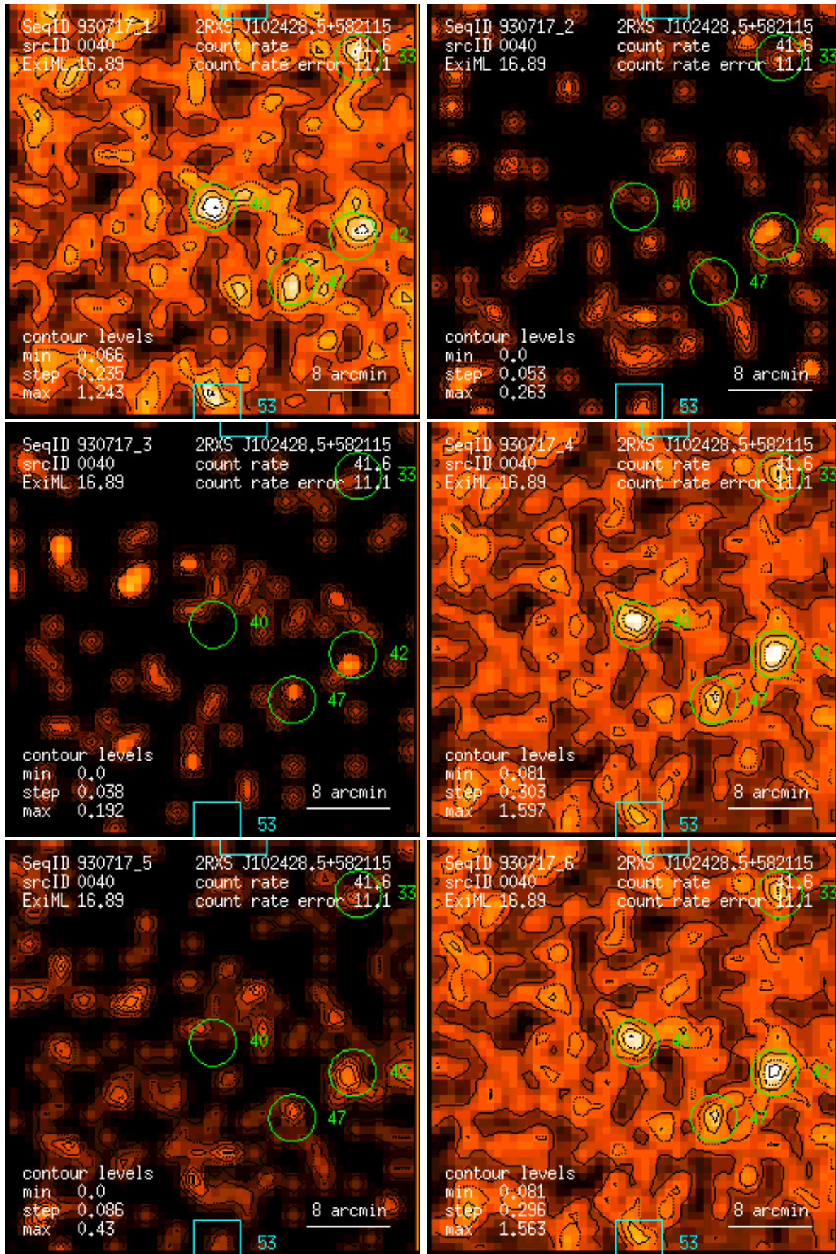
Figure 40: RASS 930717: detection 0040: band rate images, Gaussian filter: (1) PSPC channels 11 – 41, (2) 52 – 90, (3) 91 – 201, (4) 11 – 235, (5) 52 – 201, (6) 11 – 201. Broad band rates in counts/ks. Band rate contour levels in counts/ks/arcmin 2 .
