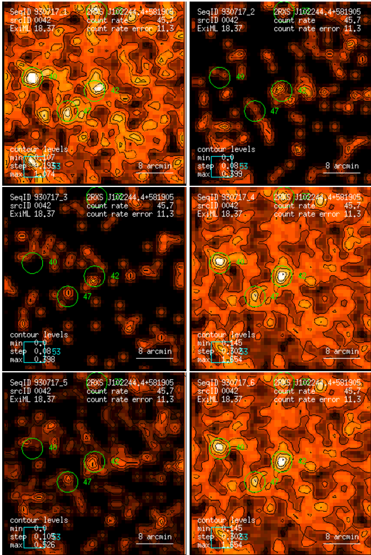
Figure 42: RASS 930717: detection 0042: band rate images, Gaussian filter: (1) PSPC channels 11 – 41, (2) 52 – 90, (3) 91 – 201, (4) 11 – 235, (5) 52 – 201, (6) 11 – 201. Broad band rates in counts/ks. Band rate contour levels in counts/ks/arcmin 2 .
