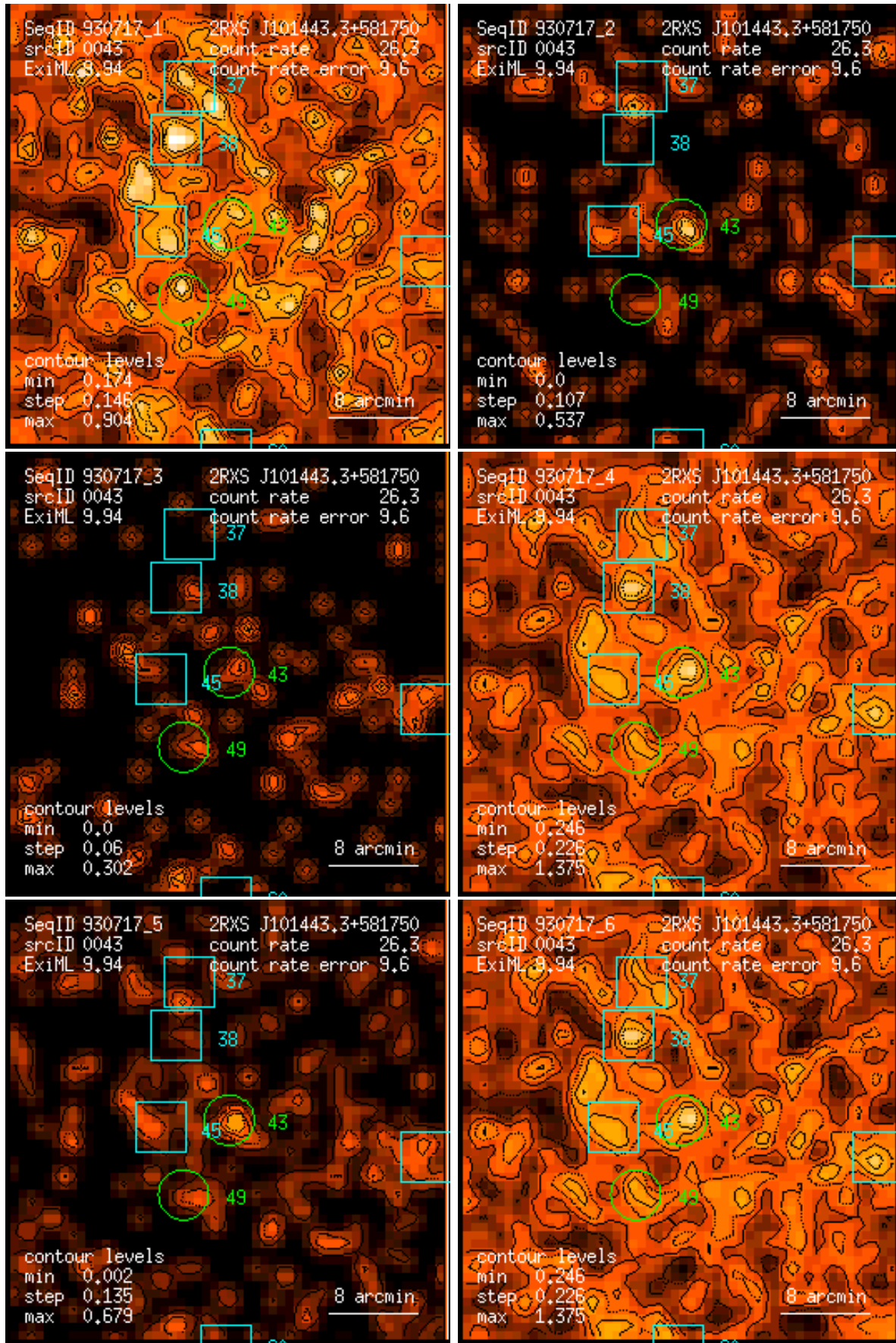
Figure 43: RASS 930717: detection 0043: band rate images, Gaussian filter: (1) PSPC channels 11 – 41, (2) 52 – 90, (3) 91 – 201, (4) 11 – 235, (5) 52 – 201, (6) 11 – 201. Broad band rates in counts/ks. Band rate contour levels in counts/ks/arcmin 2 .
