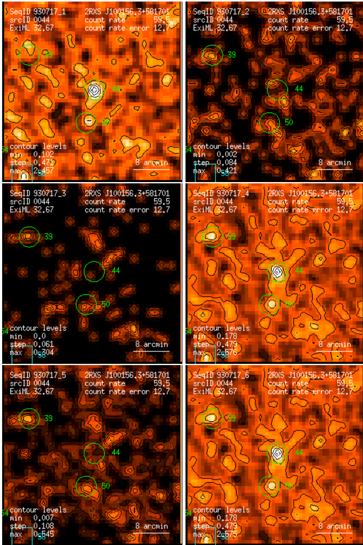
Figure 44: RASS 930717: detection 0044: band rate images, Gaussian filter: (1) PSPC channels 11 – 41, (2) 52 – 90, (3) 91 – 201, (4) 11 – 235, (5) 52 – 201, (6) 11 – 201. Broad band rates in counts/ks. Band rate contour levels in counts/ks/arcmin 2 .
