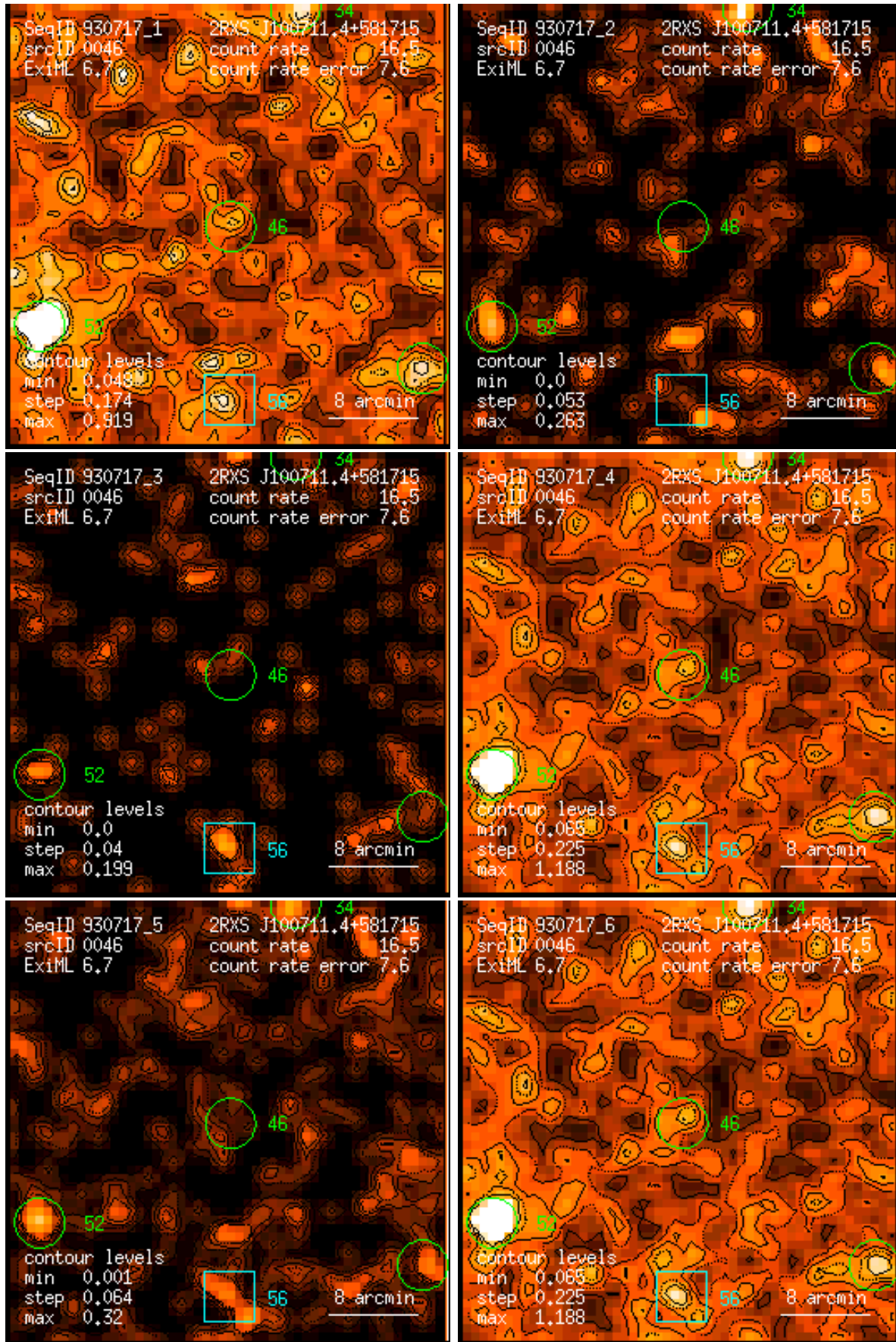
Figure 46: RASS 930717: detection 0046: band rate images, Gaussian filter: (1) PSPC channels 11 – 41, (2) 52 – 90, (3) 91 – 201, (4) 11 – 235, (5) 52 – 201, (6) 11 – 201. Broad band rates in counts/ks. Band rate contour levels in counts/ks/arcmin 2 .
