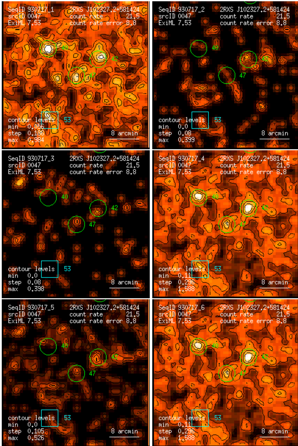
Figure 47: RASS 930717: detection 0047: band rate images, Gaussian filter: (1) PSPC channels 11 – 41, (2) 52 – 90, (3) 91 – 201, (4) 11 – 235, (5) 52 – 201, (6) 11 – 201. Broad band rates in counts/ks. Band rate contour levels in counts/ks/arcmin 2 .
