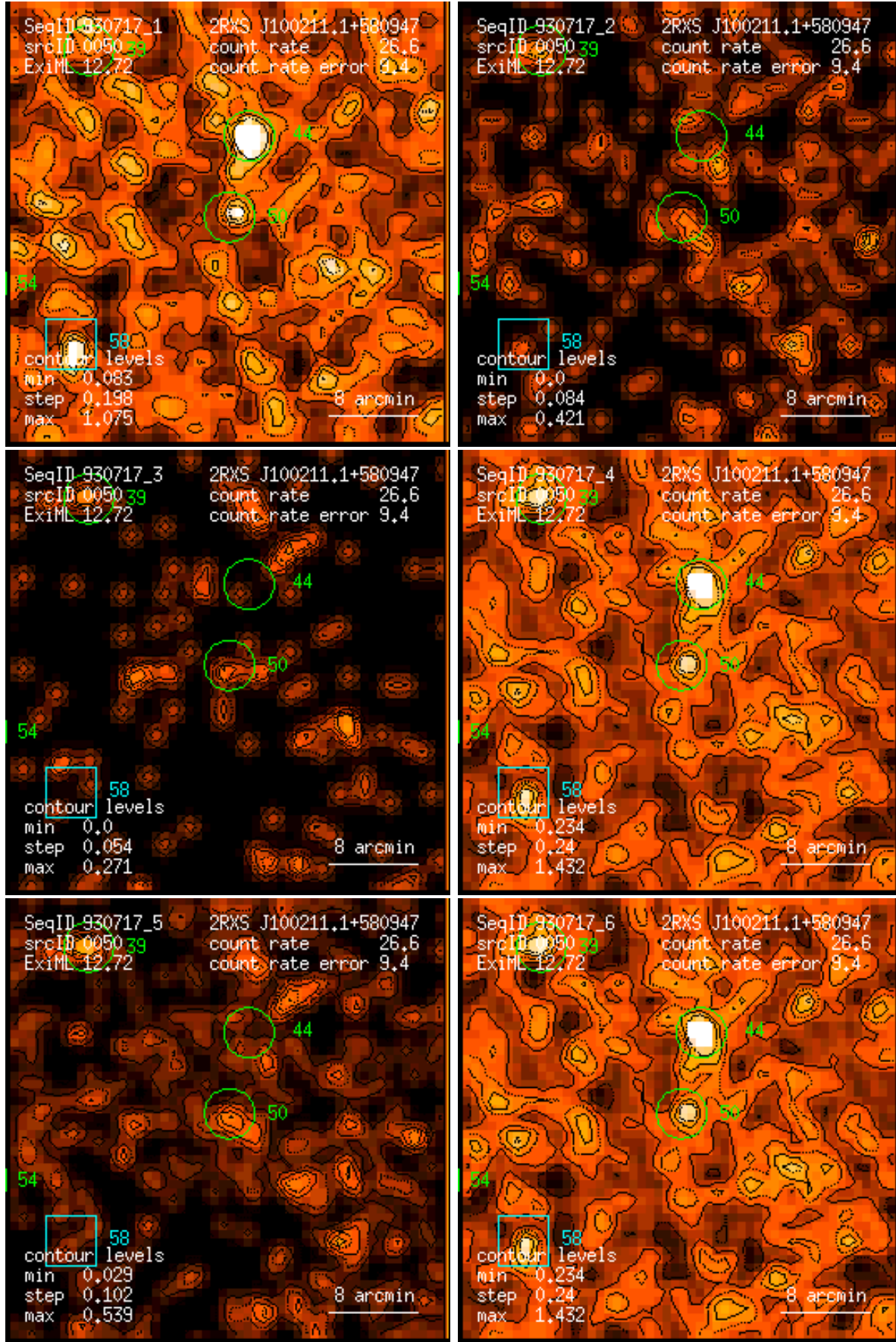
Figure 50: RASS 930717: detection 0050: band rate images, Gaussian filter: (1) PSPC channels 11 – 41, (2) 52 – 90, (3) 91 – 201, (4) 11 – 235, (5) 52 – 201, (6) 11 – 201. Broad band rates in counts/ks. Band rate contour levels in counts/ks/arcmin 2 .
