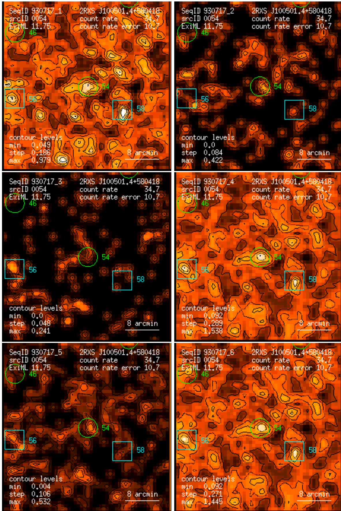
Figure 54: RASS 930717: detection 0054: band rate images, Gaussian filter: (1) PSPC channels 11 – 41, (2) 52 – 90, (3) 91 – 201, (4) 11 – 235, (5) 52 – 201, (6) 11 – 201. Broad band rates in counts/ks. Band rate contour levels in counts/ks/arcmin 2 .
