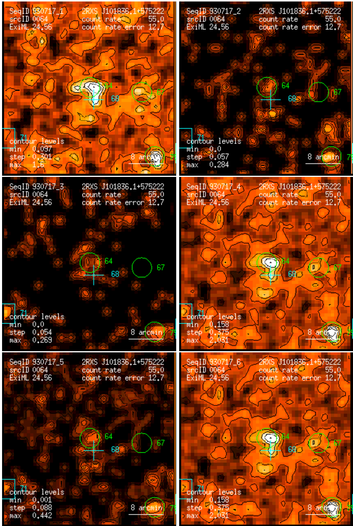
Figure 64: RASS 930717: detection 0064: band rate images, Gaussian filter: (1) PSPC channels 11 – 41, (2) 52 – 90, (3) 91 – 201, (4) 11 – 235, (5) 52 – 201, (6) 11 – 201. Broad band rates in counts/ks. Band rate contour levels in counts/ks/arcmin 2 .
