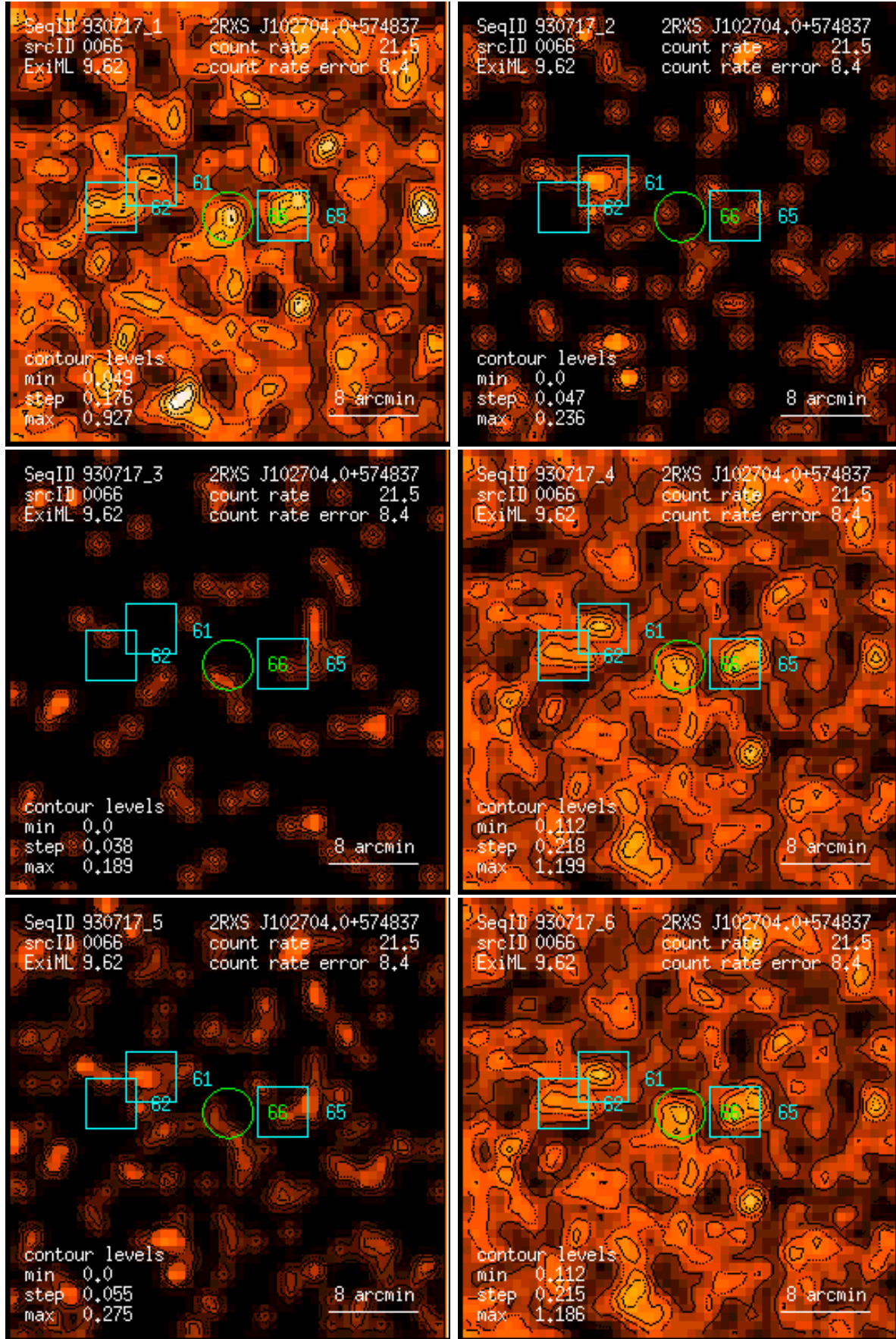
Figure 66: RASS 930717: detection 0066: band rate images, Gaussian filter: (1) PSPC channels 11 – 41, (2) 52 – 90, (3) 91 – 201, (4) 11 – 235, (5) 52 – 201, (6) 11 – 201. Broad band rates in counts/ks. Band rate contour levels in counts/ks/arcmin 2 .
