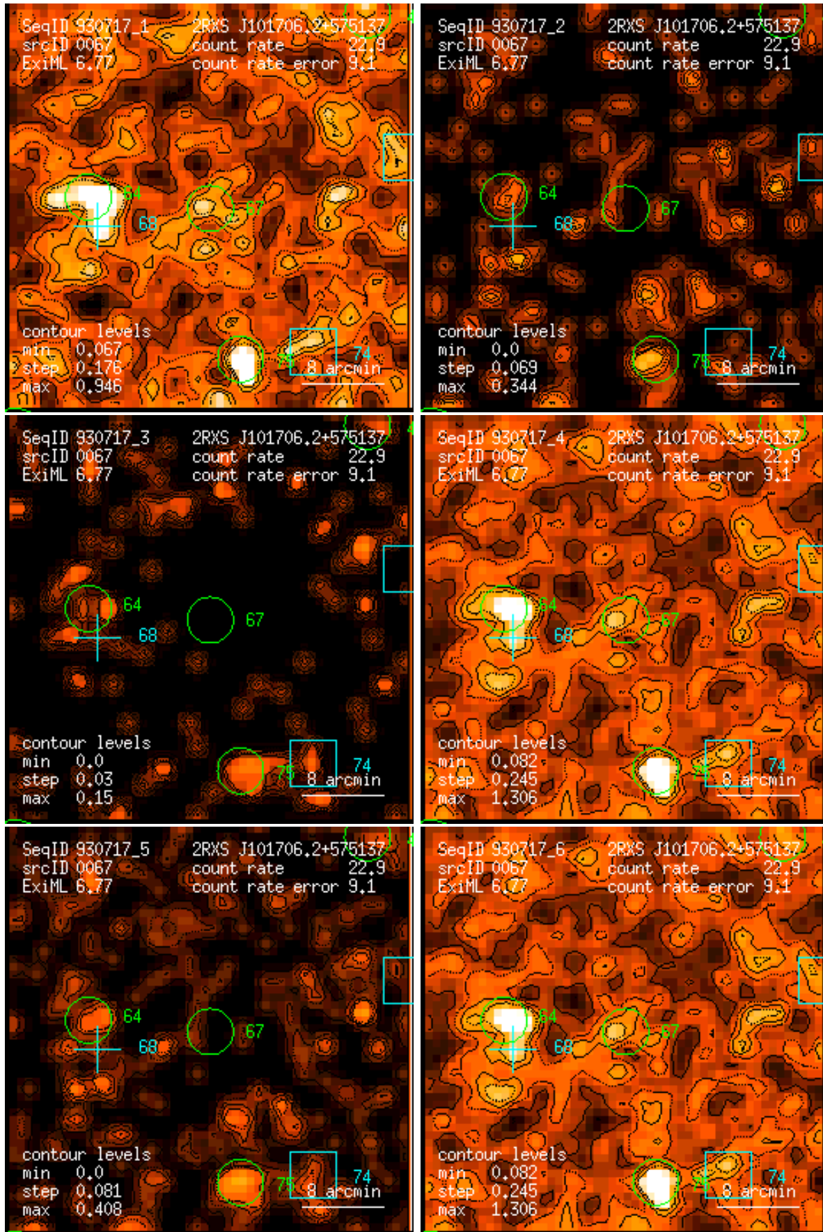
Figure 67: RASS 930717: detection 0067: band rate images, Gaussian filter: (1) PSPC channels 11 – 41, (2) 52 – 90, (3) 91 – 201, (4) 11 – 235, (5) 52 – 201, (6) 11 – 201. Broad band rates in counts/ks. Band rate contour levels in counts/ks/arcmin 2 .
