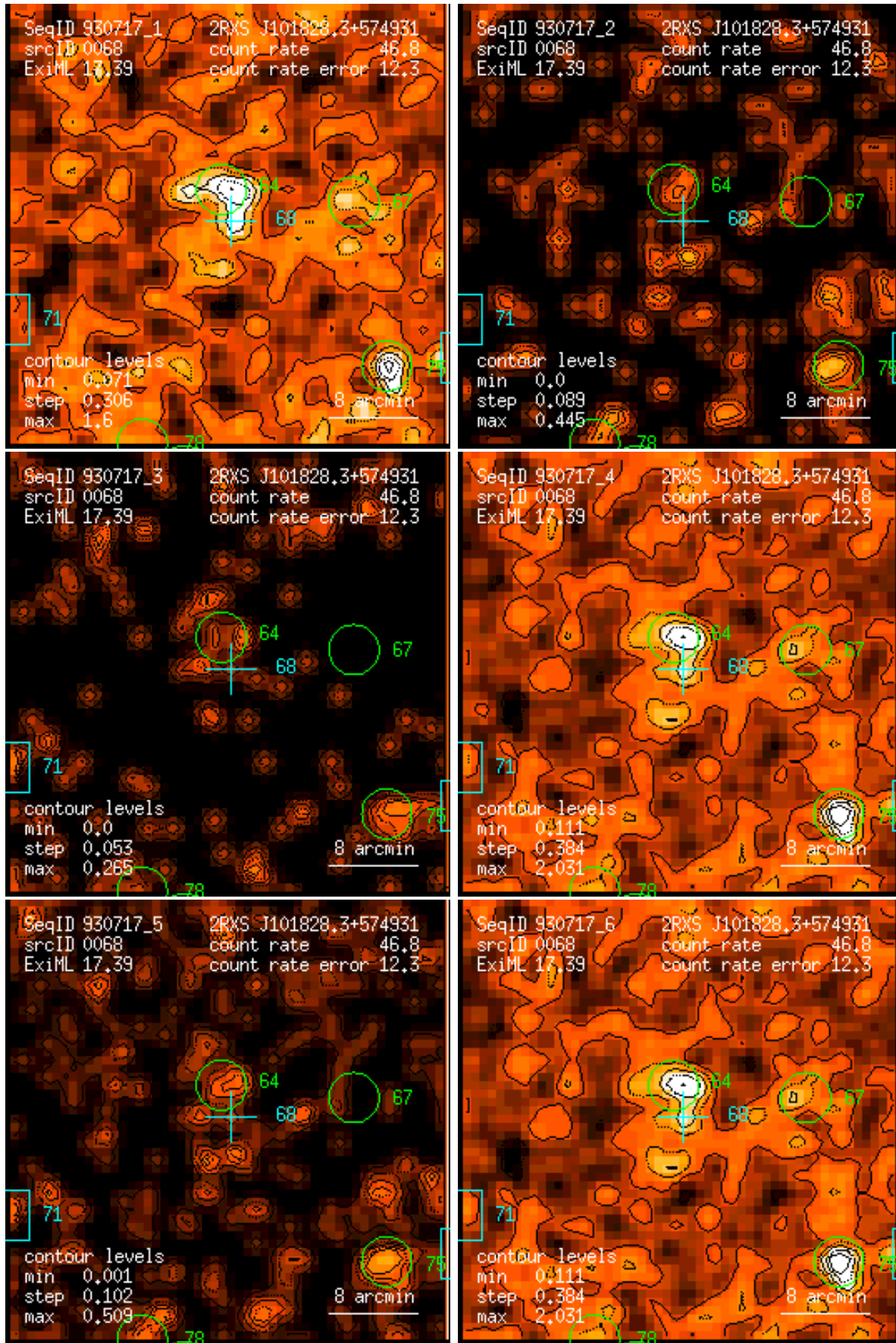
Figure 68: RASS 930717: detection 0068: band rate images, Gaussian filter: (1) PSPC channels 11 – 41, (2) 52 – 90, (3) 91 – 201, (4) 11 – 235, (5) 52 – 201, (6) 11 – 201. Broad band rates in counts/ks. Band rate contour levels in counts/ks/arcmin 2 .
