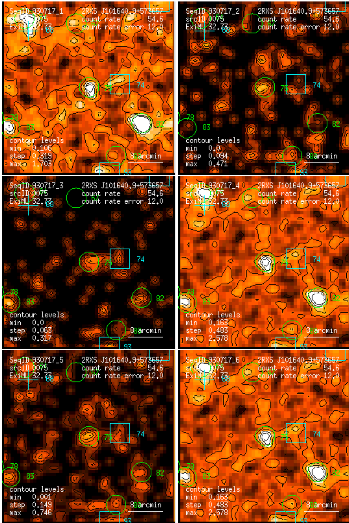
Figure 75: RASS 930717: detection 0075: band rate images, Gaussian filter: (1) PSPC channels 11 – 41, (2) 52 – 90, (3) 91 – 201, (4) 11 – 235, (5) 52 – 201, (6) 11 – 201. Broad band rates in counts/ks. Band rate contour levels in counts/ks/arcmin 2 .
