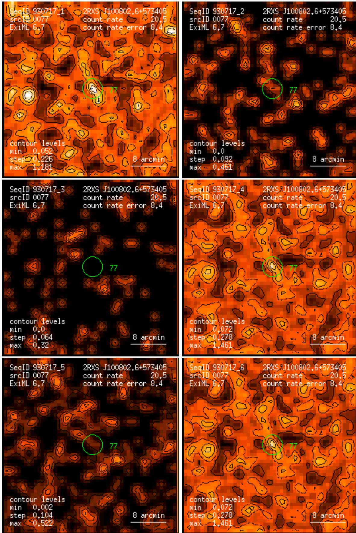
Figure 77: RASS 930717: detection 0077: band rate images, Gaussian filter: (1) PSPC channels 11 – 41, (2) 52 – 90, (3) 91 – 201, (4) 11 – 235, (5) 52 – 201, (6) 11 – 201. Broad band rates in counts/ks. Band rate contour levels in counts/ks/arcmin 2 .
