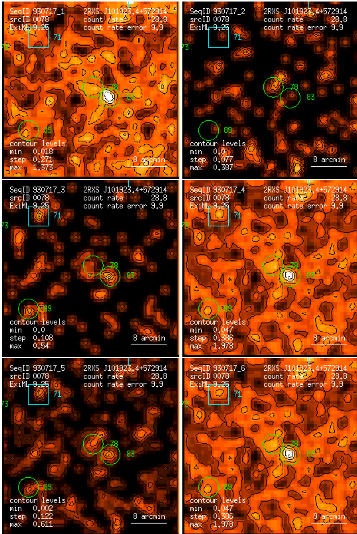
Figure 78: RASS 930717: detection 0078: band rate images, Gaussian filter: (1) PSPC channels 11 – 41, (2) 52 – 90, (3) 91 – 201, (4) 11 – 235, (5) 52 – 201, (6) 11 – 201. Broad band rates in counts/ks. Band rate contour levels in counts/ks/arcmin 2 .
