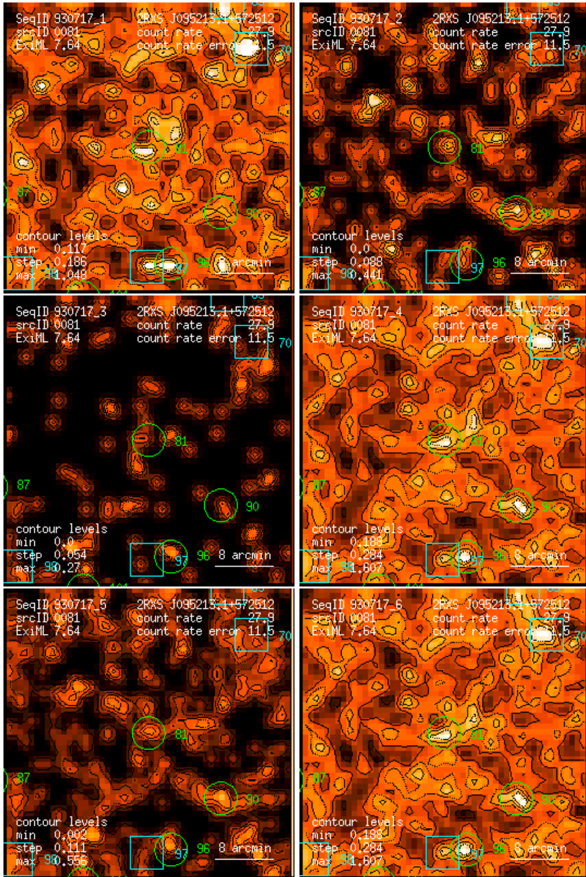
Figure 81: RASS 930717: detection 0081: band rate images, Gaussian filter: (1) PSPC channels 11 – 41, (2) 52 – 90, (3) 91 – 201, (4) 11 – 235, (5) 52 – 201, (6) 11 – 201. Broad band rates in counts/ks. Band rate contour levels in counts/ks/arcmin 2 .
