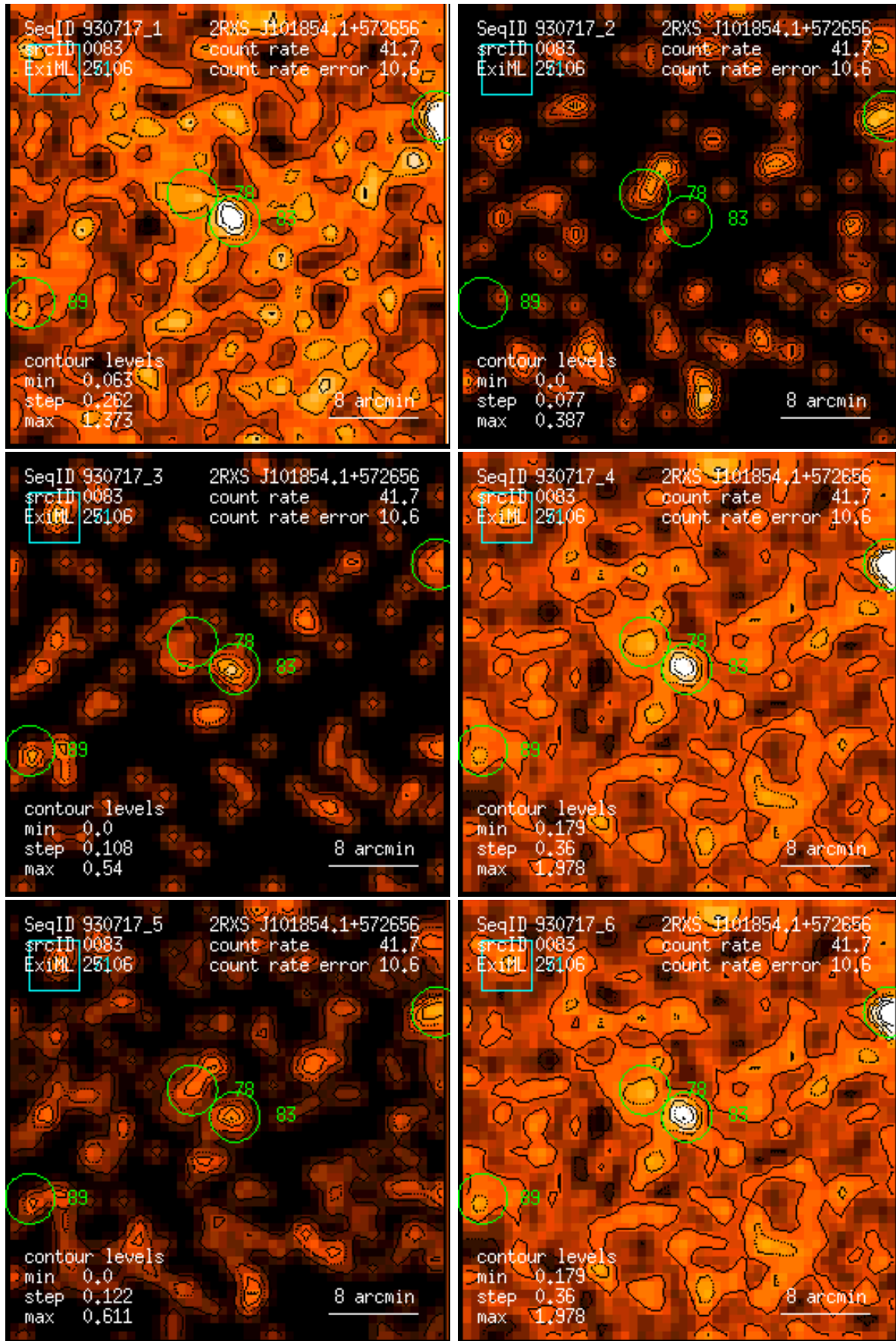
Figure 83: RASS 930717: detection 0083: band rate images, Gaussian filter: (1) PSPC channels 11 – 41, (2) 52 – 90, (3) 91 – 201, (4) 11 – 235, (5) 52 – 201, (6) 11 – 201. Broad band rates in counts/ks. Band rate contour levels in counts/ks/arcmin 2 .
