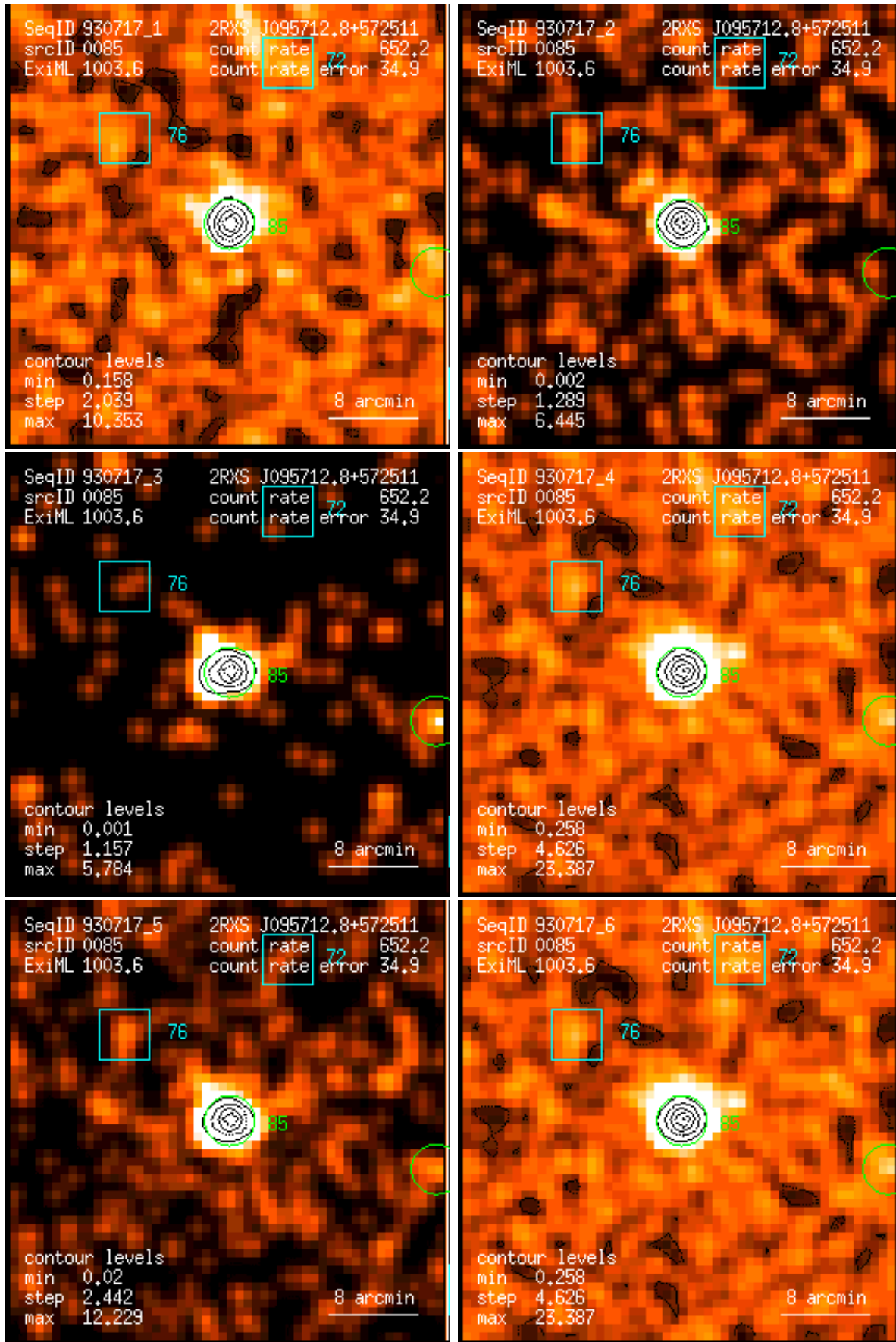
Figure 85: RASS 930717: detection 0085: band rate images, Gaussian filter: (1) PSPC channels 11 – 41, (2) 52 – 90, (3) 91 – 201, (4) 11 – 235, (5) 52 – 201, (6) 11 – 201. Broad band rates in counts/ks. Band rate contour levels in counts/ks/arcmin 2 .
