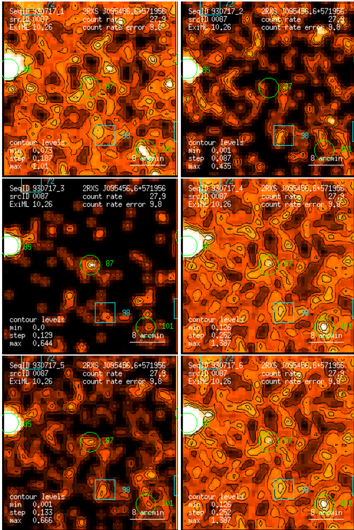
Figure 87: RASS 930717: detection 0087: band rate images, Gaussian filter: (1) PSPC channels 11 – 41, (2) 52 – 90, (3) 91 – 201, (4) 11 – 235, (5) 52 – 201, (6) 11 – 201. Broad band rates in counts/ks. Band rate contour levels in counts/ks/arcmin 2 .
