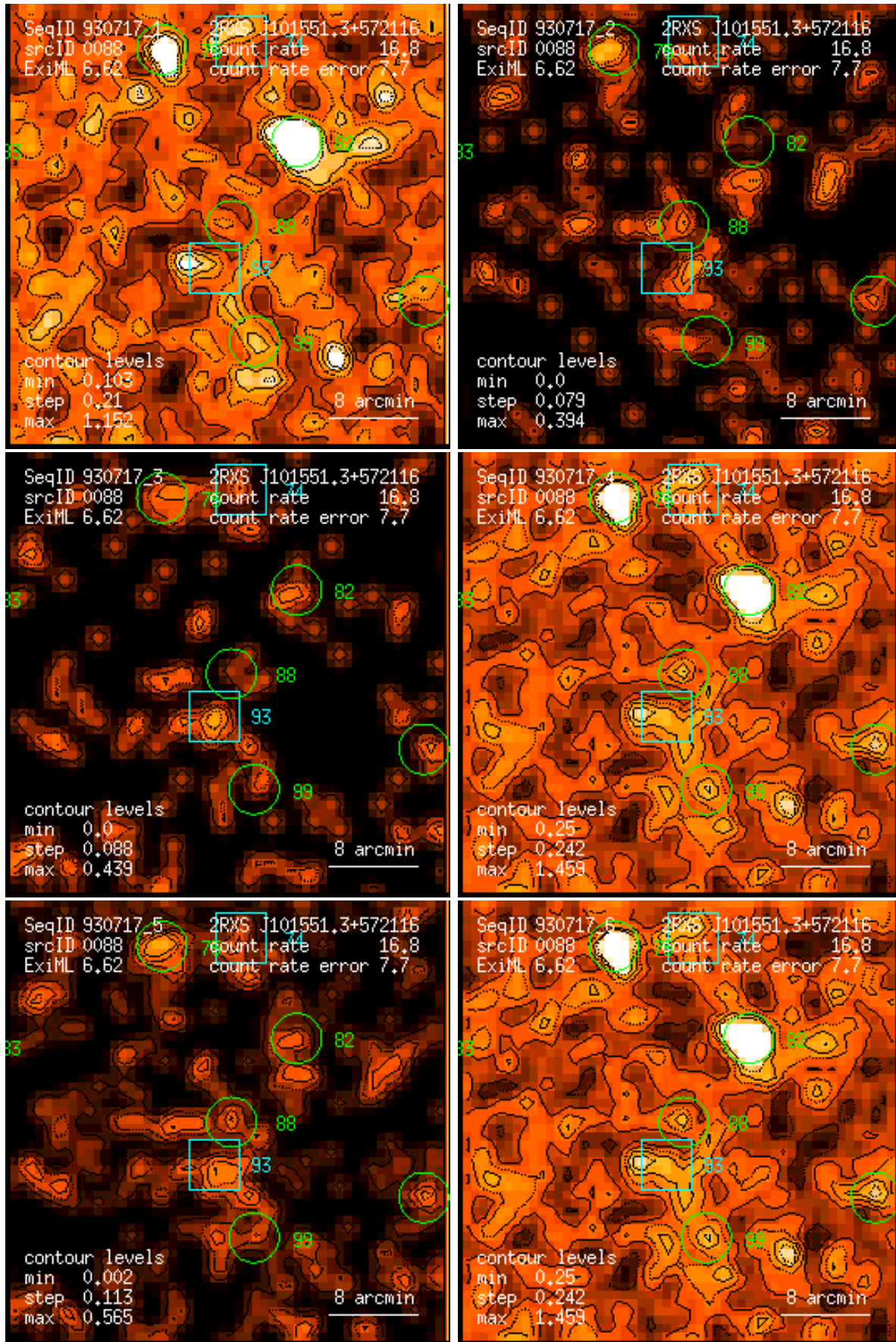
Figure 88: RASS 930717: detection 0088: band rate images, Gaussian filter: (1) PSPC channels 11 – 41, (2) 52 – 90, (3) 91 – 201, (4) 11 – 235, (5) 52 – 201, (6) 11 – 201. Broad band rates in counts/ks. Band rate contour levels in counts/ks/arcmin 2 .
