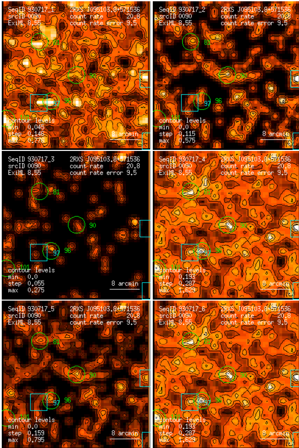
Figure 90: RASS 930717: detection 0090: band rate images, Gaussian filter: (1) PSPC channels 11 – 41, (2) 52 – 90, (3) 91 – 201, (4) 11 – 235, (5) 52 – 201, (6) 11 – 201. Broad band rates in counts/ks. Band rate contour levels in counts/ks/arcmin 2 .
