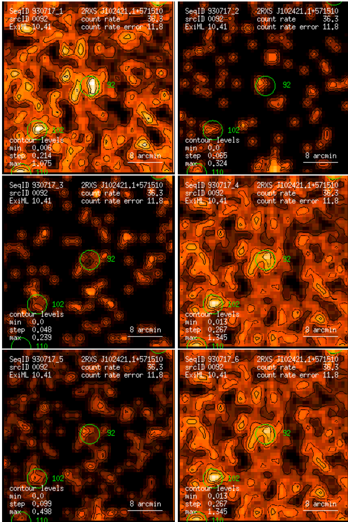
Figure 92: RASS 930717: detection 0092: band rate images, Gaussian filter: (1) PSPC channels 11 – 41, (2) 52 – 90, (3) 91 – 201, (4) 11 – 235, (5) 52 – 201, (6) 11 – 201. Broad band rates in counts/ks. Band rate contour levels in counts/ks/arcmin 2 .
