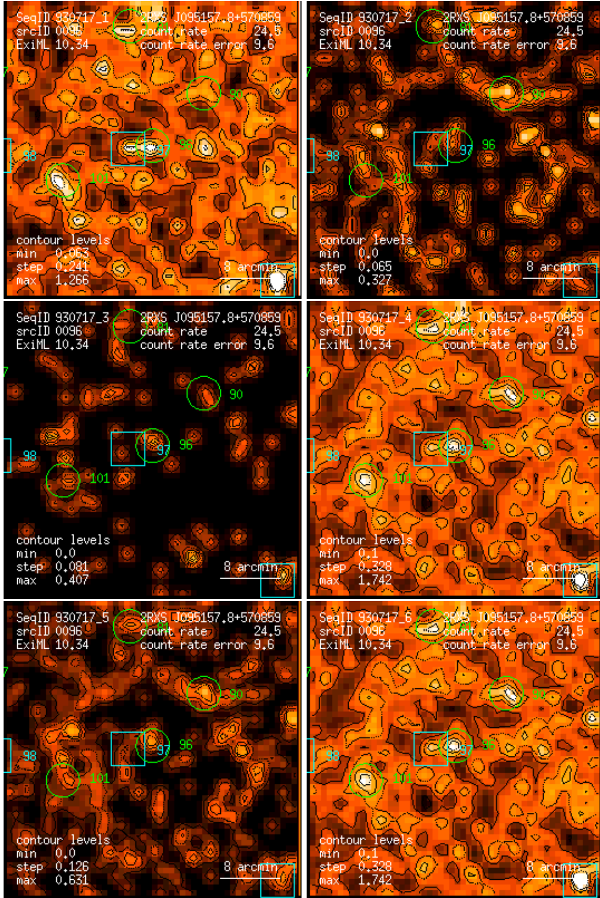
Figure 96: RASS 930717: detection 0096: band rate images, Gaussian filter: (1) PSPC channels 11 – 41, (2) 52 – 90, (3) 91 – 201, (4) 11 – 235, (5) 52 – 201, (6) 11 – 201. Broad band rates in counts/ks. Band rate contour levels in counts/ks/arcmin 2 .
