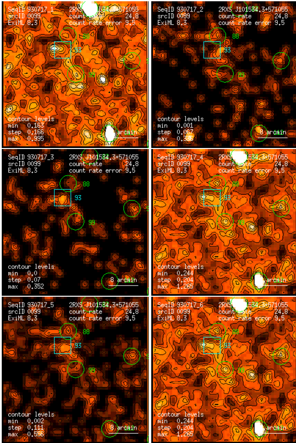
Figure 99: RASS 930717: detection 0099: band rate images, Gaussian filter: (1) PSPC channels 11 – 41, (2) 52 – 90, (3) 91 – 201, (4) 11 – 235, (5) 52 – 201, (6) 11 – 201. Broad band rates in counts/ks. Band rate contour levels in counts/ks/arcmin 2 .
