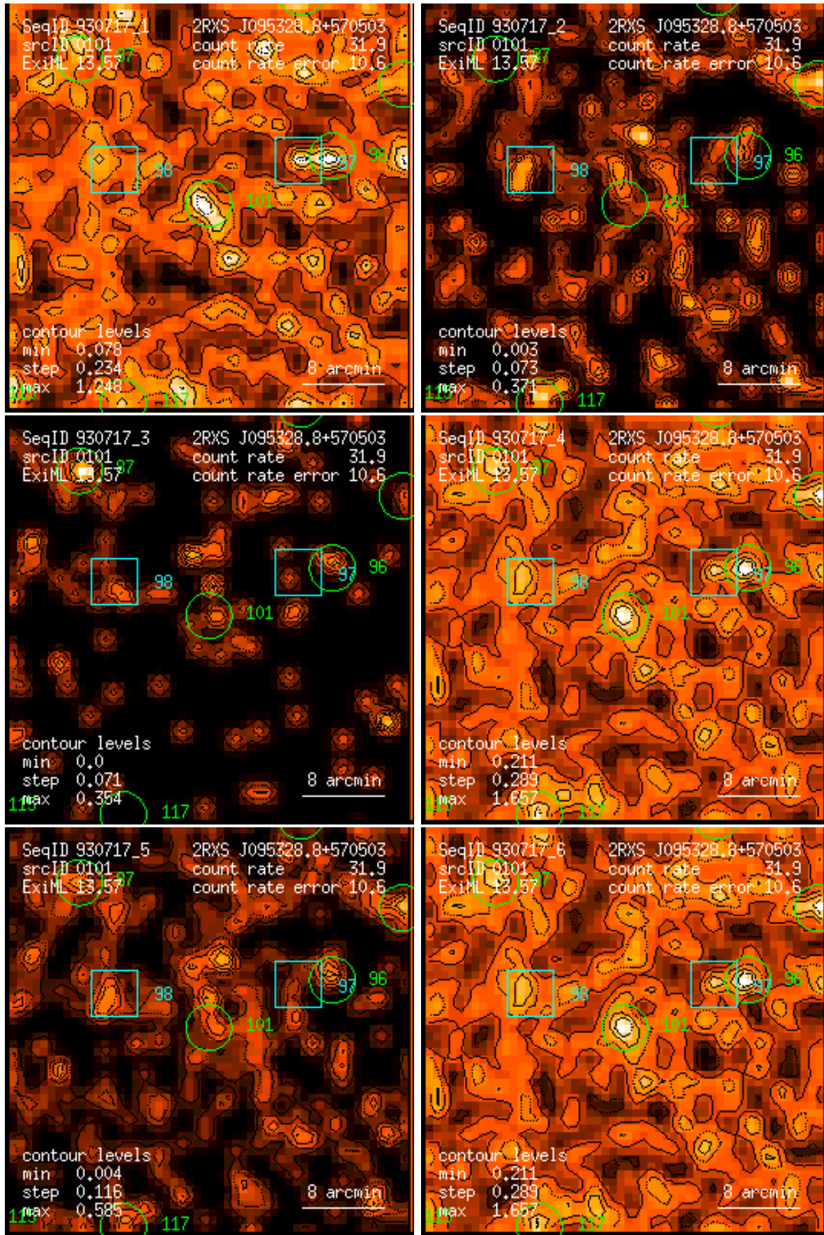
Figure 101: RASS 930717: detection 0101: band rate images, Gaussian filter: (1) PSPC channels 11 – 41, (2) 52 – 90, (3) 91 – 201, (4) 11 – 235, (5) 52 – 201, (6) 11 – 201. Broad band rates in counts/ks. Band rate contour levels in counts/ks/arcmin 2 .
