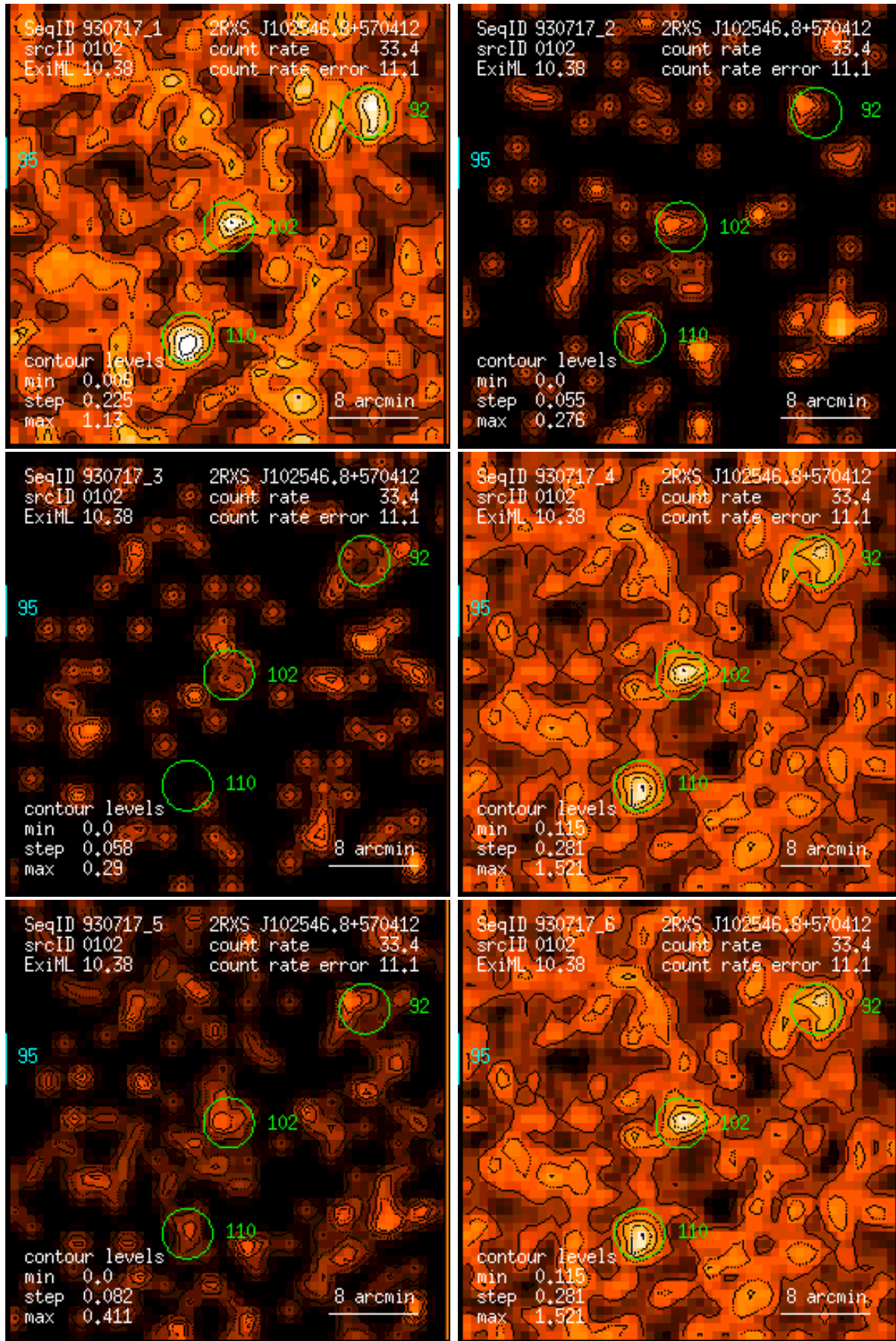
Figure 102: RASS 930717: detection 0102: band rate images, Gaussian filter: (1) PSPC channels 11 – 41, (2) 52 – 90, (3) 91 – 201, (4) 11 – 235, (5) 52 – 201, (6) 11 – 201. Broad band rates in counts/ks. Band rate contour levels in counts/ks/arcmin 2 .
