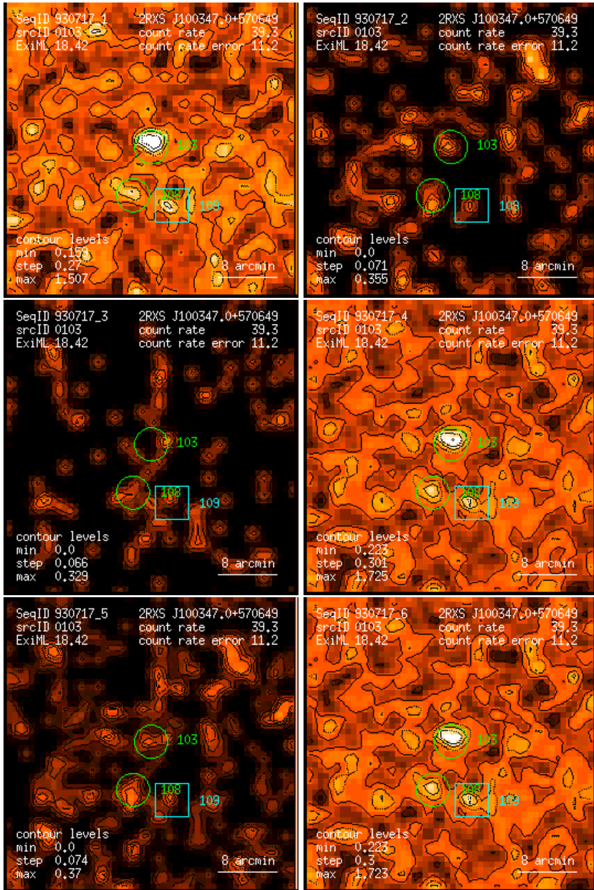
Figure 103: RASS 930717: detection 0103: band rate images, Gaussian filter: (1) PSPC channels 11 – 41, (2) 52 – 90, (3) 91 – 201, (4) 11 – 235, (5) 52 – 201, (6) 11 – 201. Broad band rates in counts/ks. Band rate contour levels in counts/ks/arcmin 2 .
