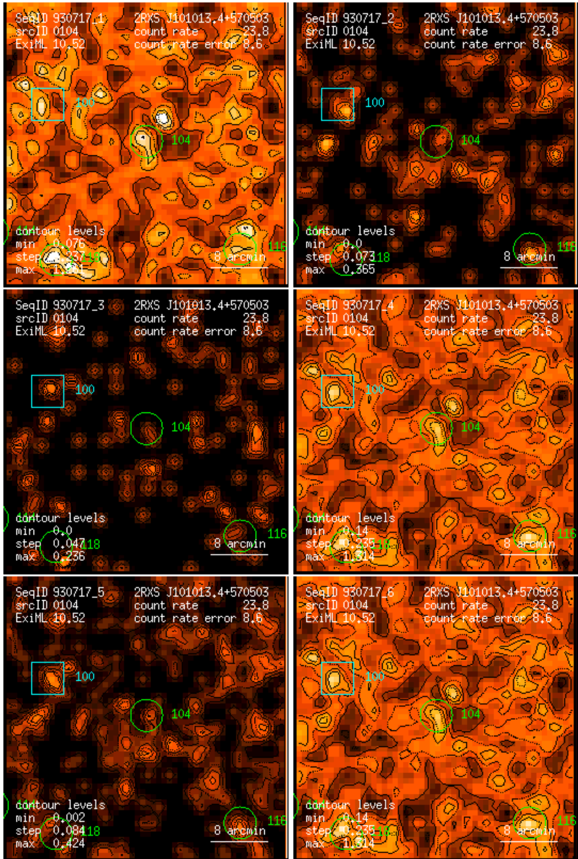
Figure 104: RASS 930717: detection 0104: band rate images, Gaussian filter: (1) PSPC channels 11 – 41, (2) 52 – 90, (3) 91 – 201, (4) 11 – 235, (5) 52 – 201, (6) 11 – 201. Broad band rates in counts/ks. Band rate contour levels in counts/ks/arcmin 2 .
