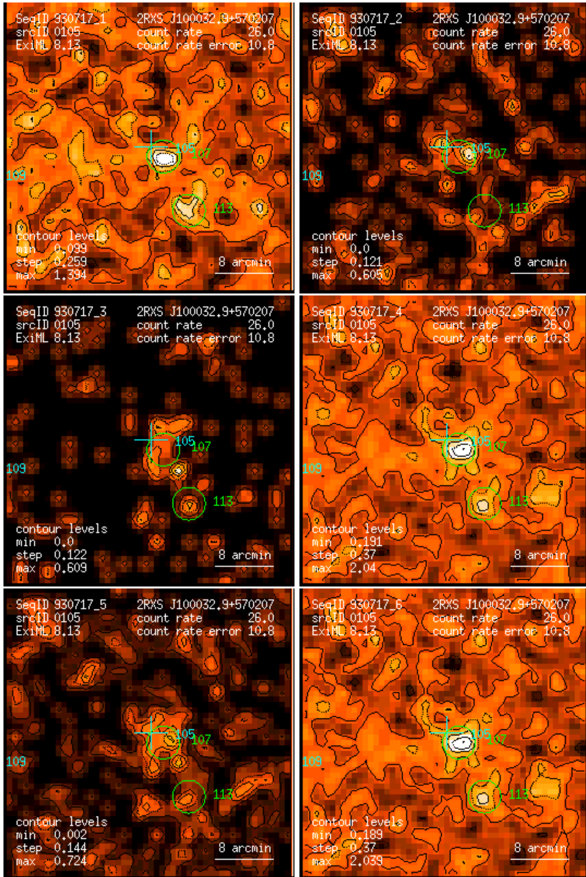
Figure 105: RASS 930717: detection 0105: band rate images, Gaussian filter: (1) PSPC channels 11 – 41, (2) 52 – 90, (3) 91 – 201, (4) 11 – 235, (5) 52 – 201, (6) 11 – 201. Broad band rates in counts/ks. Band rate contour levels in counts/ks/arcmin 2 .
