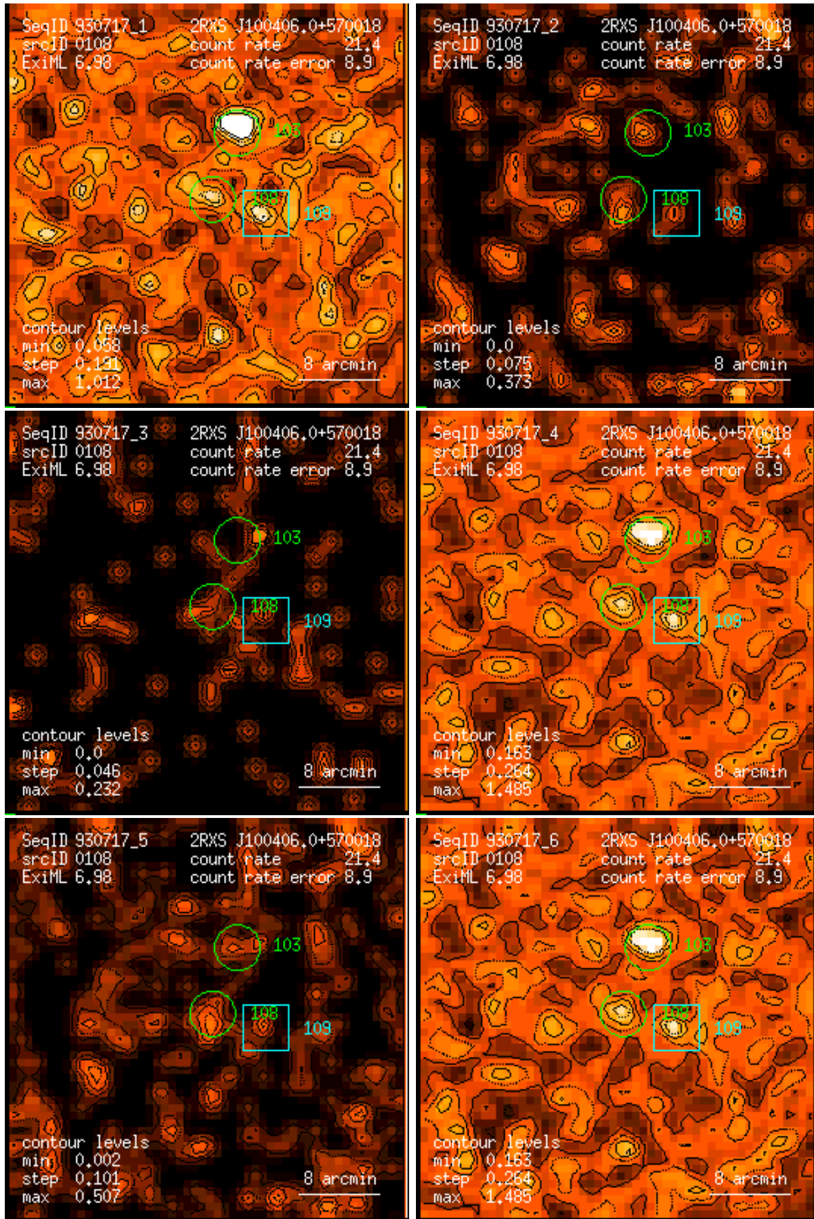
Figure 108: RASS 930717: detection 0108: band rate images, Gaussian filter: (1) PSPC channels 11 – 41, (2) 52 – 90, (3) 91 – 201, (4) 11 – 235, (5) 52 – 201, (6) 11 – 201. Broad band rates in counts/ks. Band rate contour levels in counts/ks/arcmin 2 .
