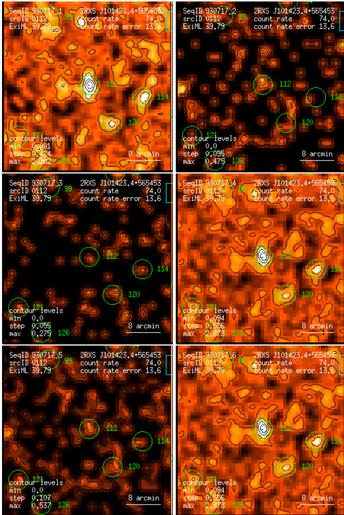
Figure 112: RASS 930717: detection 0112: band rate images, Gaussian filter: (1) PSPC channels 11 – 41, (2) 52 – 90, (3) 91 – 201, (4) 11 – 235, (5) 52 – 201, (6) 11 – 201. Broad band rates in counts/ks. Band rate contour levels in counts/ks/arcmin 2 .
