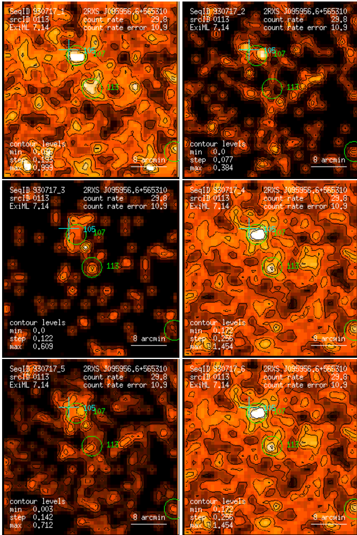
Figure 113: RASS 930717: detection 0113: band rate images, Gaussian filter: (1) PSPC channels 11 – 41, (2) 52 – 90, (3) 91 – 201, (4) 11 – 235, (5) 52 – 201, (6) 11 – 201. Broad band rates in counts/ks. Band rate contour levels in counts/ks/arcmin 2 .
