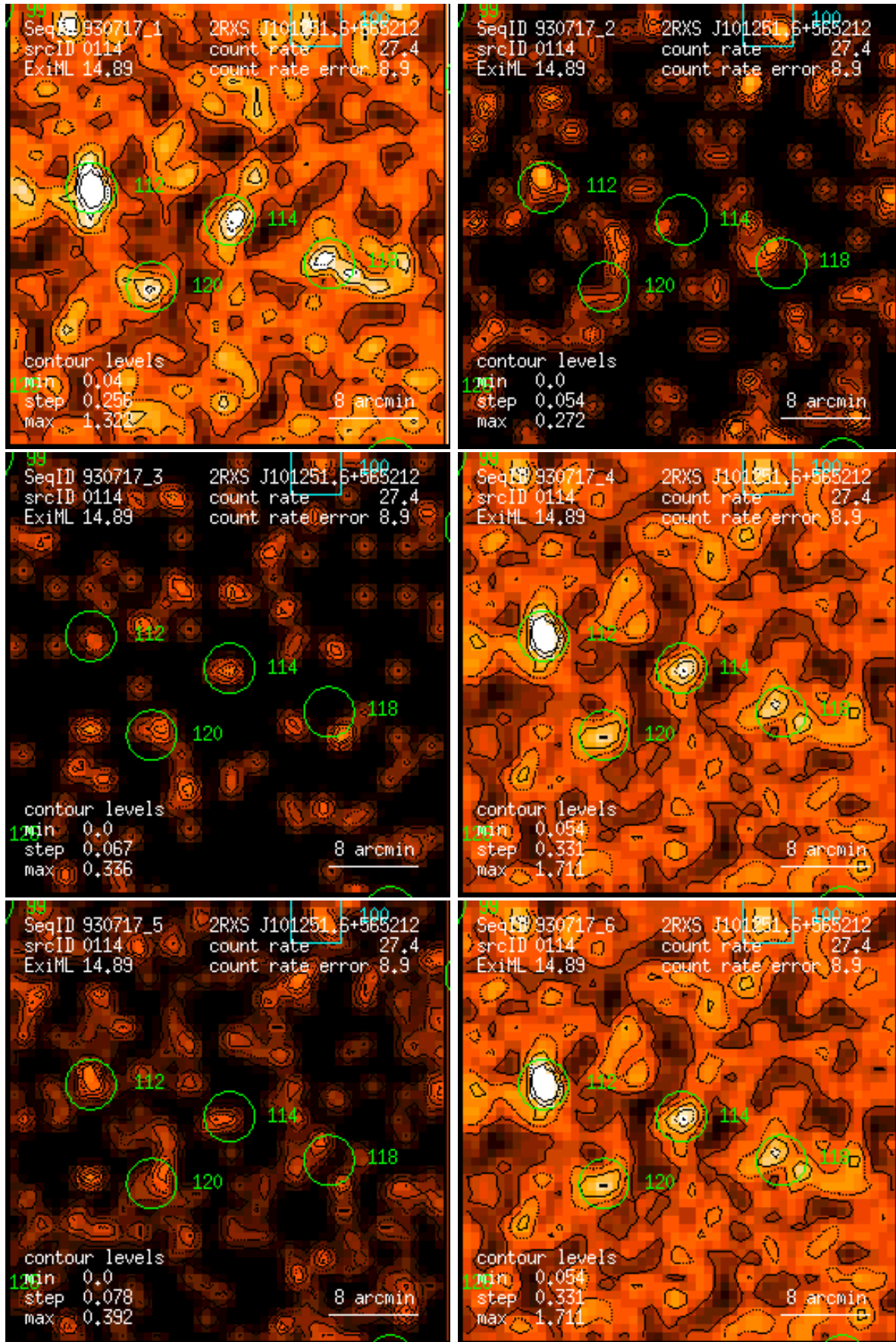
Figure 114: RASS 930717: detection 0114: band rate images, Gaussian filter: (1) PSPC channels 11 – 41, (2) 52 – 90, (3) 91 – 201, (4) 11 – 235, (5) 52 – 201, (6) 11 – 201. Broad band rates in counts/ks. Band rate contour levels in counts/ks/arcmin 2 .
