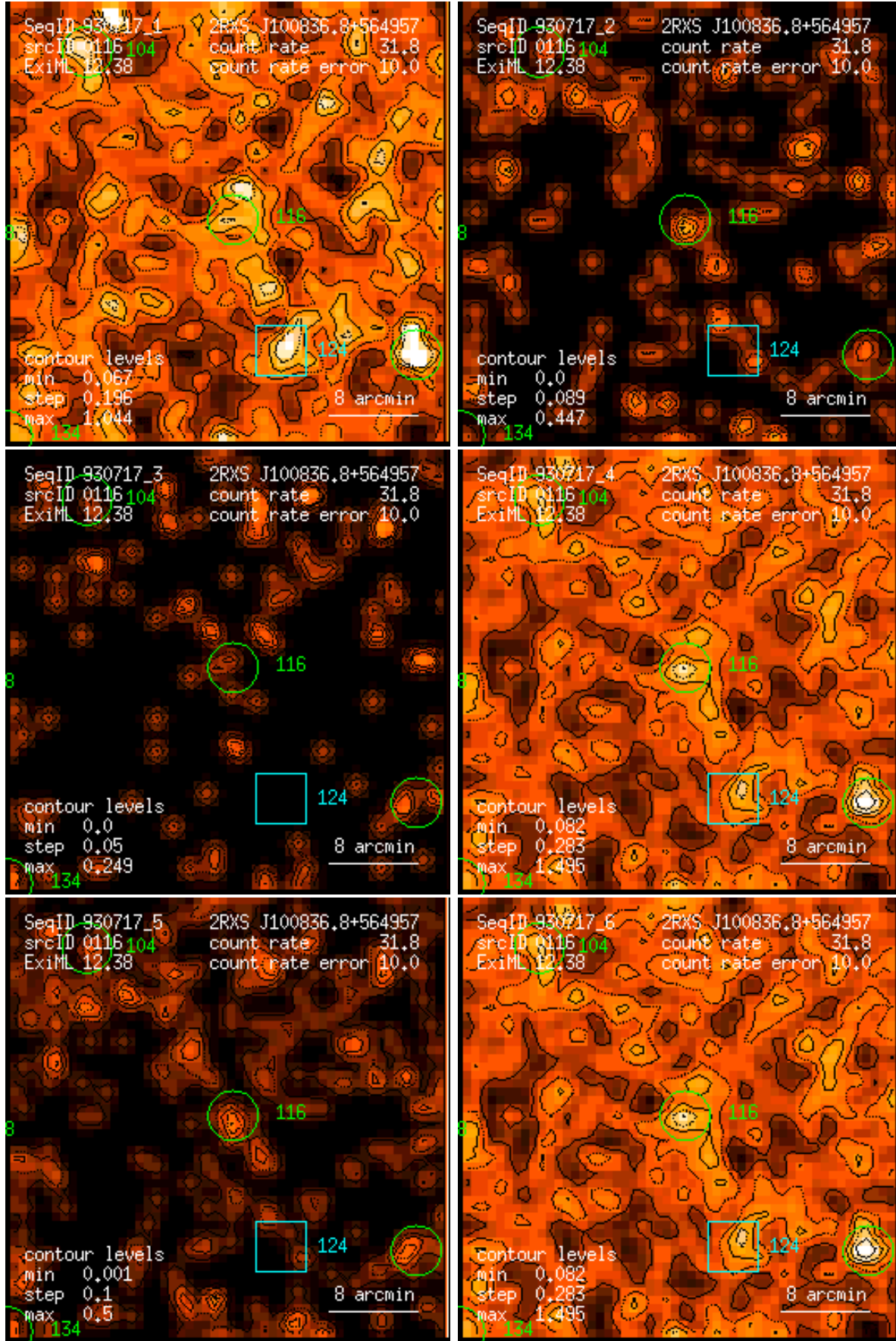
Figure 116: RASS 930717: detection 0116: band rate images, Gaussian filter: (1) PSPC channels 11 – 41, (2) 52 – 90, (3) 91 – 201, (4) 11 – 235, (5) 52 – 201, (6) 11 – 201. Broad band rates in counts/ks. Band rate contour levels in counts/ks/arcmin 2 .
