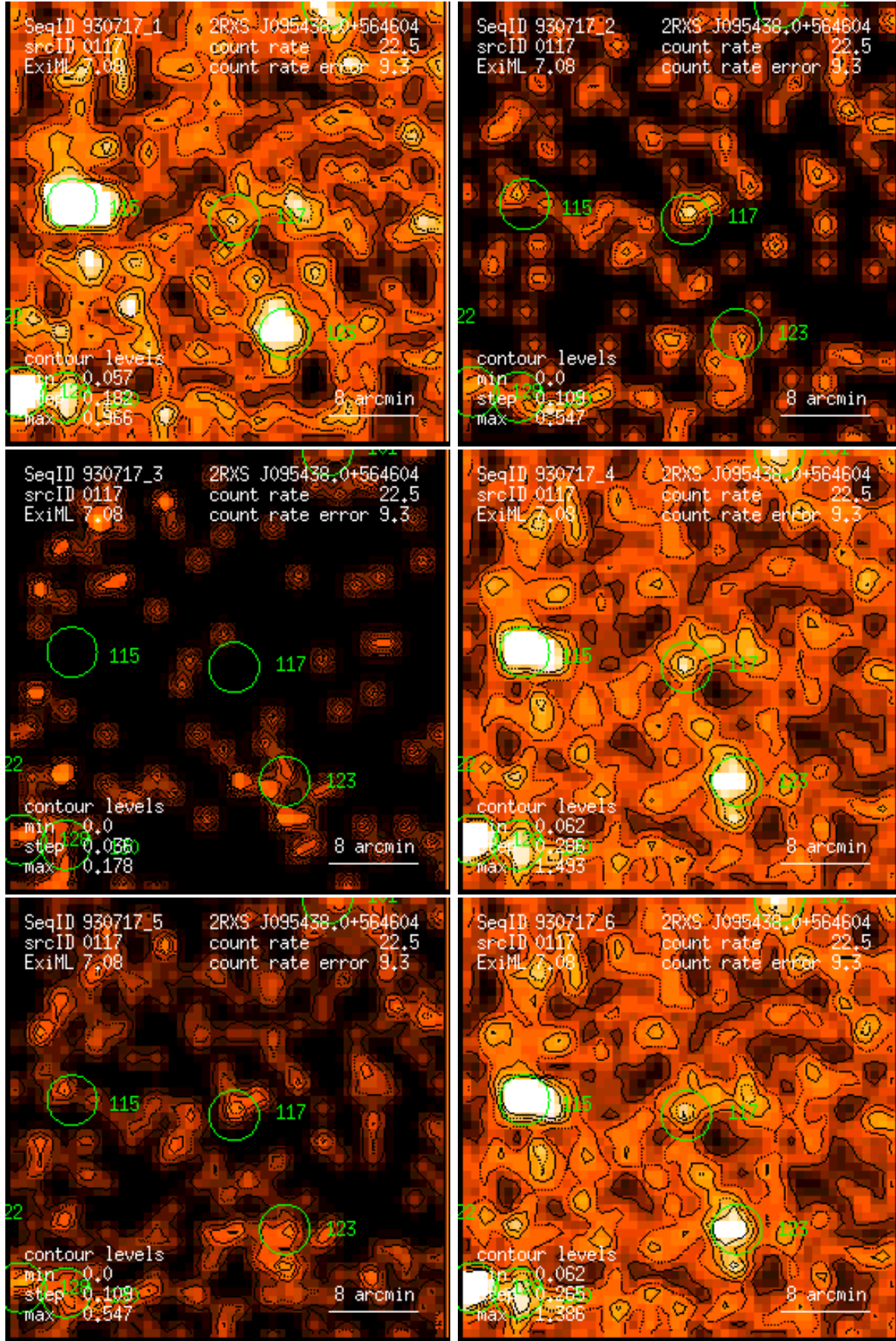
Figure 117: RASS 930717: detection 0117: band rate images, Gaussian filter: (1) PSPC channels 11 – 41, (2) 52 – 90, (3) 91 – 201, (4) 11 – 235, (5) 52 – 201, (6) 11 – 201. Broad band rates in counts/ks. Band rate contour levels in counts/ks/arcmin 2 .
