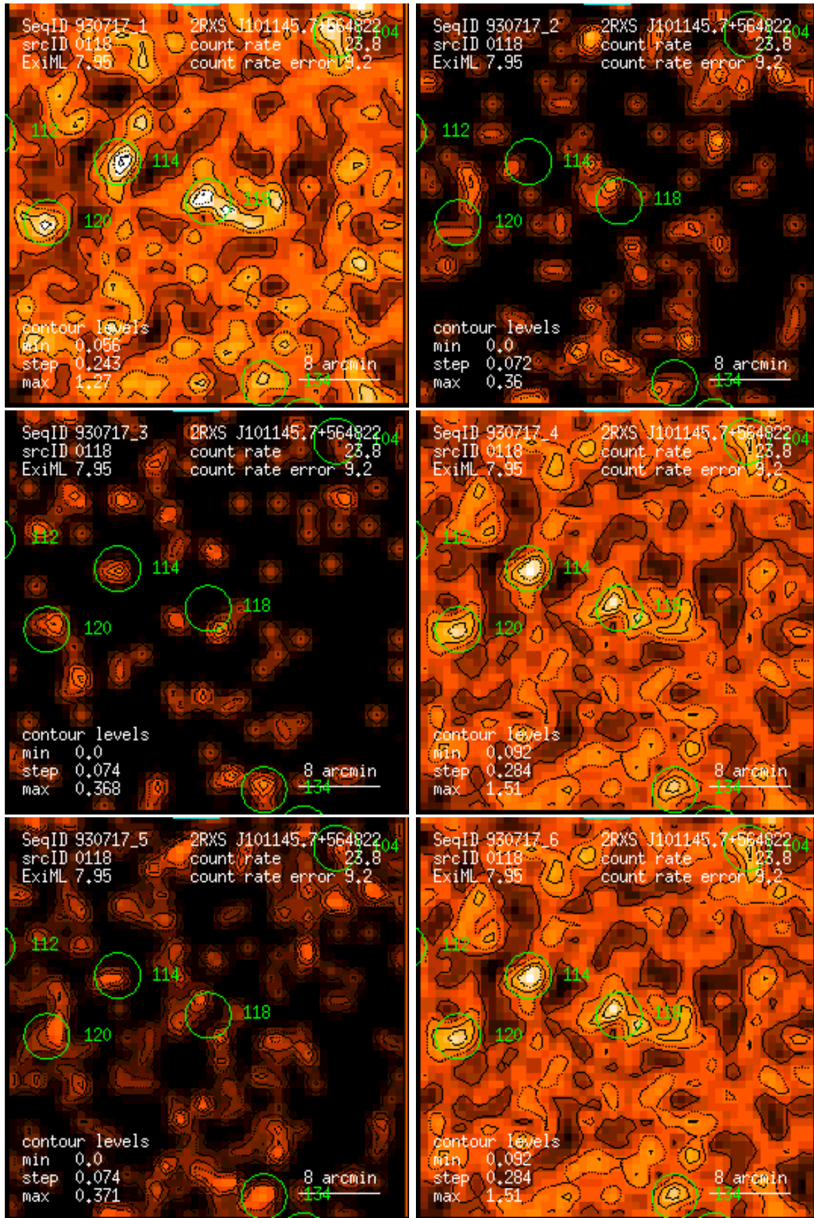
Figure 118: RASS 930717: detection 0118: band rate images, Gaussian filter: (1) PSPC channels 11 – 41, (2) 52 – 90, (3) 91 – 201, (4) 11 – 235, (5) 52 – 201, (6) 11 – 201. Broad band rates in counts/ks. Band rate contour levels in counts/ks/arcmin 2 .
