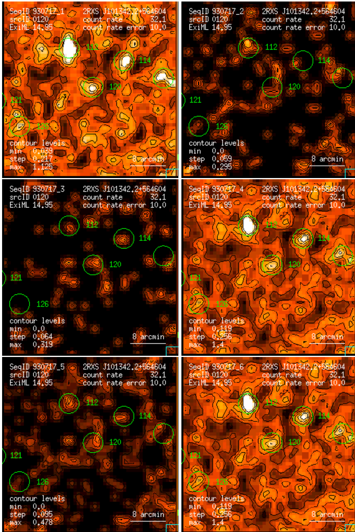
Figure 120: RASS 930717: detection 0120: band rate images, Gaussian filter: (1) PSPC channels 11 – 41, (2) 52 – 90, (3) 91 – 201, (4) 11 – 235, (5) 52 – 201, (6) 11 – 201. Broad band rates in counts/ks. Band rate contour levels in counts/ks/arcmin 2 .
