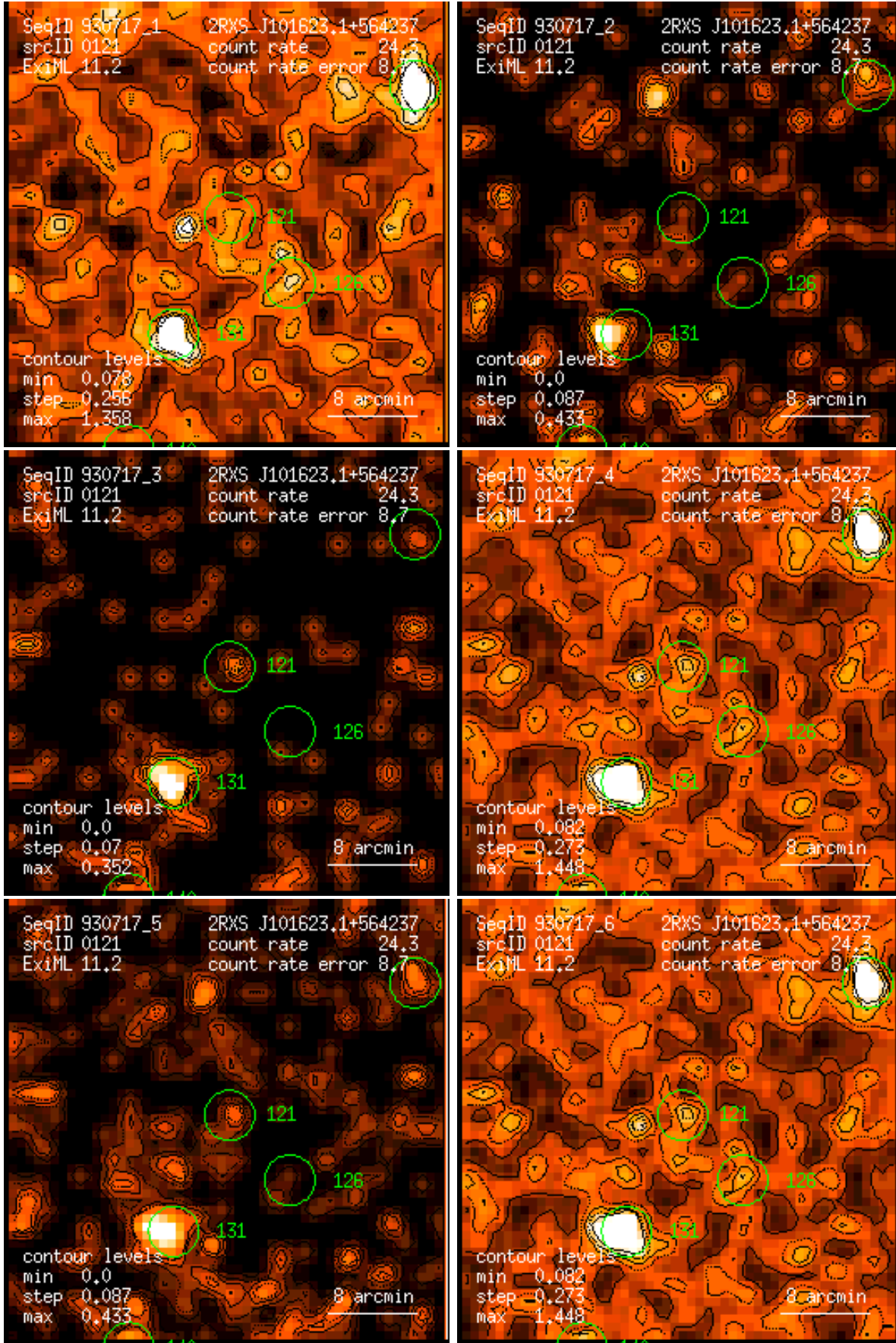
Figure 121: RASS 930717: detection 0121: band rate images, Gaussian filter: (1) PSPC channels 11 – 41, (2) 52 – 90, (3) 91 – 201, (4) 11 – 235, (5) 52 – 201, (6) 11 – 201. Broad band rates in counts/ks. Band rate contour levels in counts/ks/arcmin 2 .
