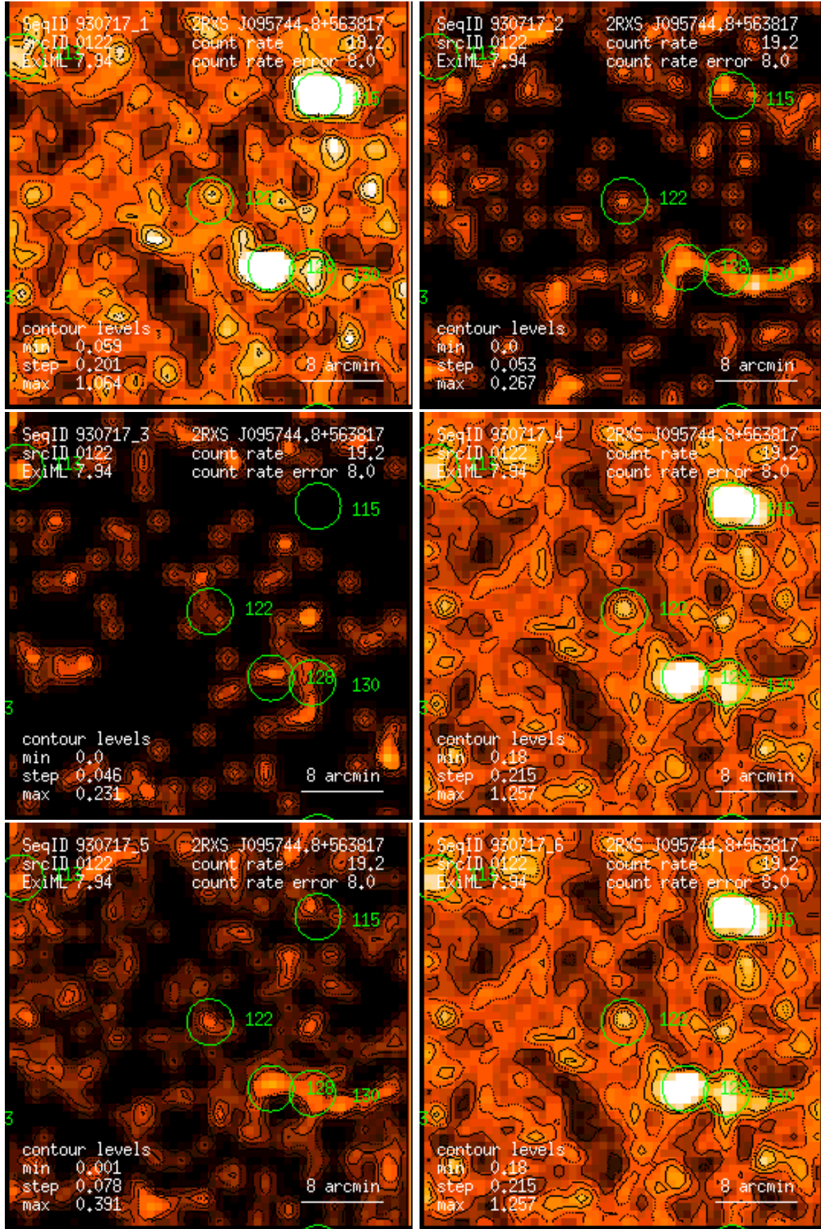
Figure 122: RASS 930717: detection 0122: band rate images, Gaussian filter: (1) PSPC channels 11 – 41, (2) 52 – 90, (3) 91 – 201, (4) 11 – 235, (5) 52 – 201, (6) 11 – 201. Broad band rates in counts/ks. Band rate contour levels in counts/ks/arcmin 2 .
