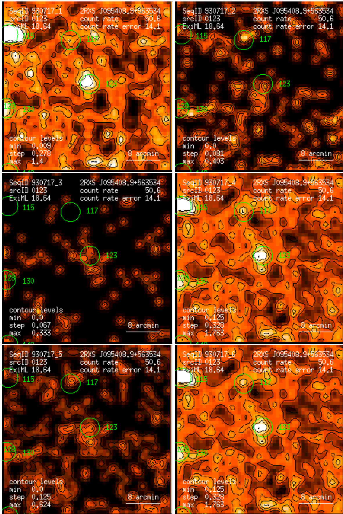
Figure 123: RASS 930717: detection 0123: band rate images, Gaussian filter: (1) PSPC channels 11 – 41, (2) 52 – 90, (3) 91 – 201, (4) 11 – 235, (5) 52 – 201, (6) 11 – 201. Broad band rates in counts/ks. Band rate contour levels in counts/ks/arcmin 2 .
