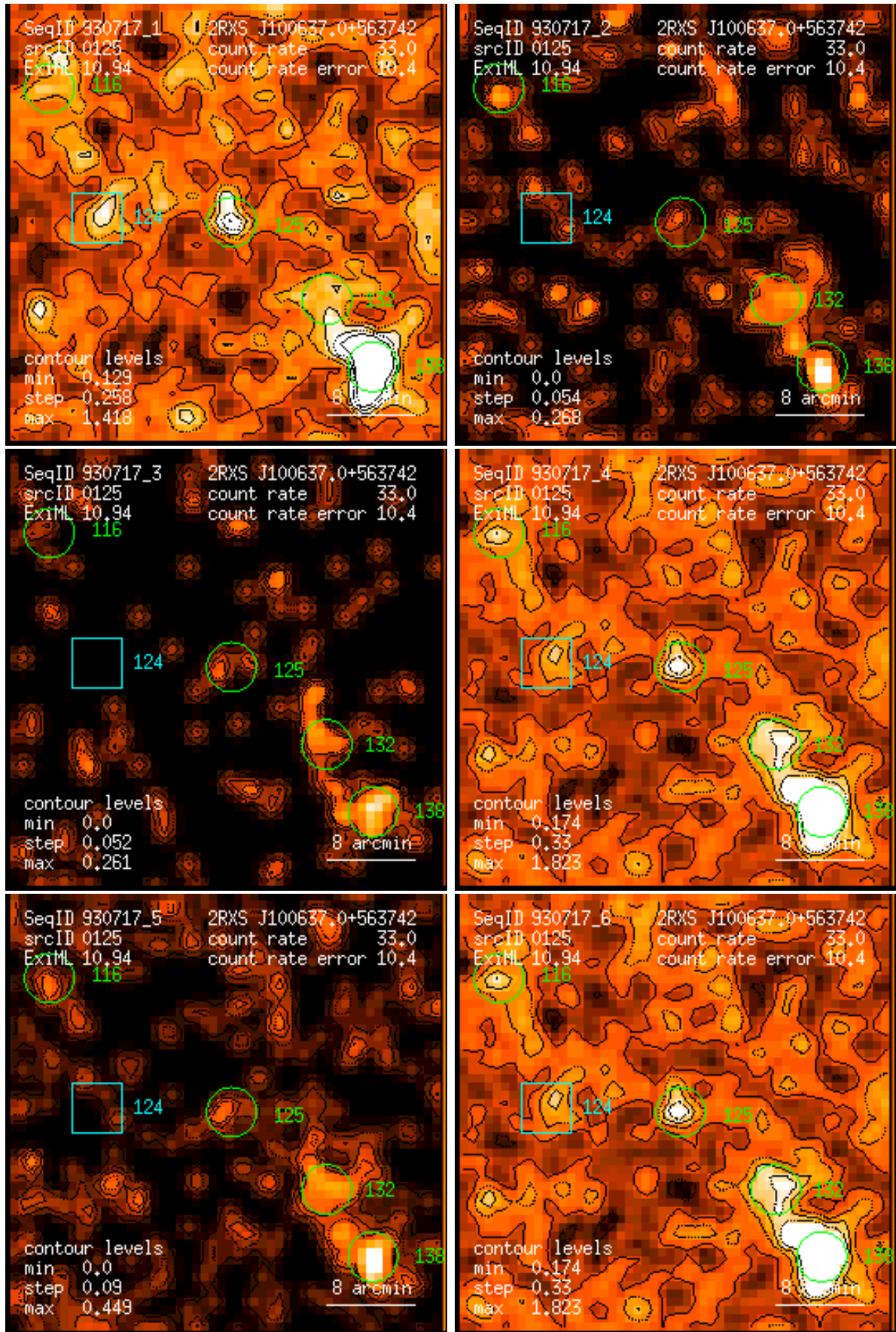
Figure 125: RASS 930717: detection 0125: band rate images, Gaussian filter: (1) PSPC channels 11 – 41, (2) 52 – 90, (3) 91 – 201, (4) 11 – 235, (5) 52 – 201, (6) 11 – 201. Broad band rates in counts/ks. Band rate contour levels in counts/ks/arcmin 2 .
